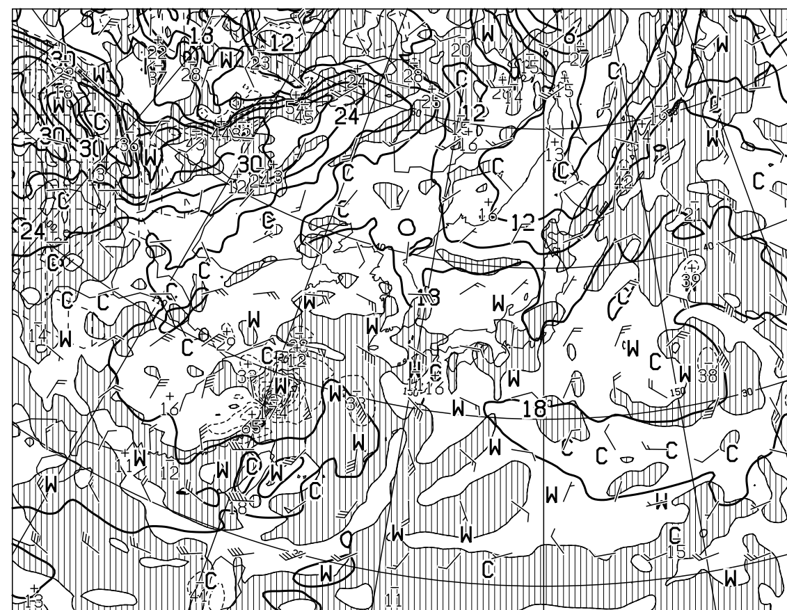
T=24 VALID 091200UTC TEMP (C), WIND ARROW AT 850hPa P-VEL (hPa/H) AT 700hPa
