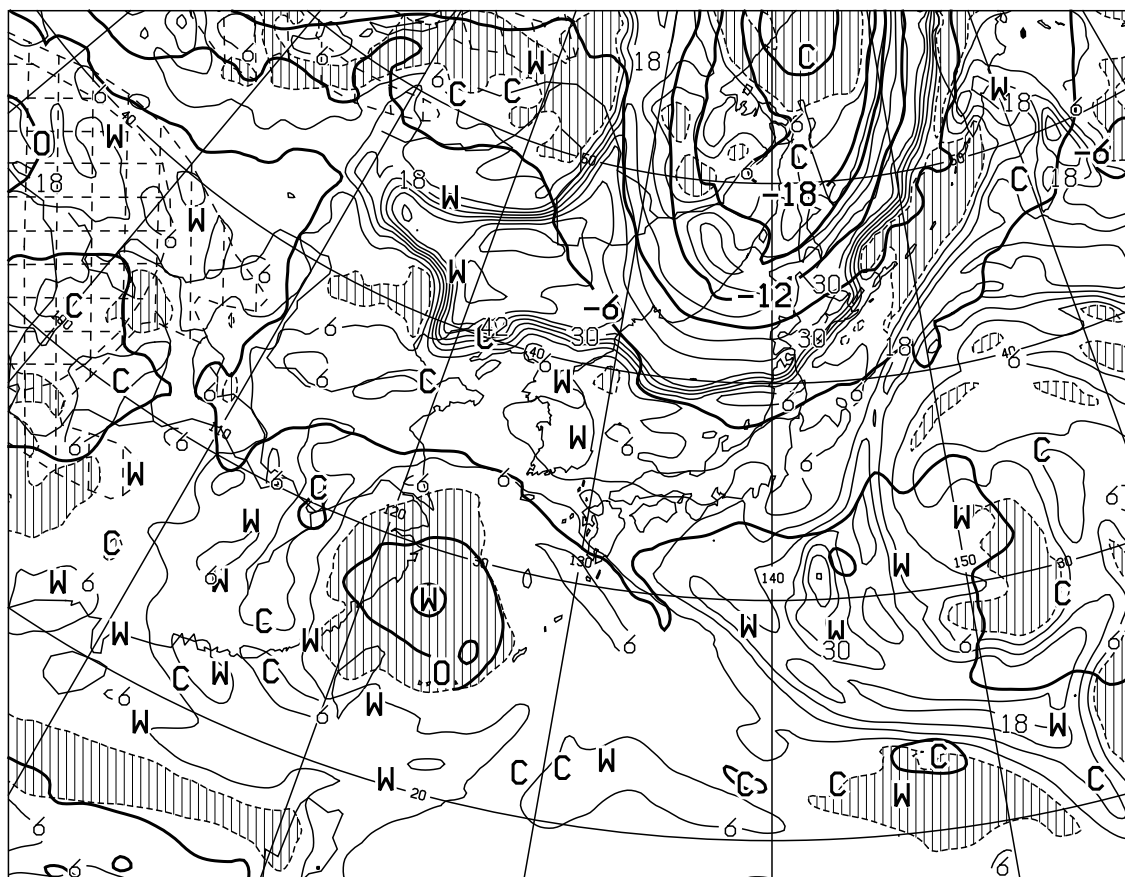
T=12 VALID 090000UTC TEMP (C) AT 500hPa T-TD (C) AT 700hPa
