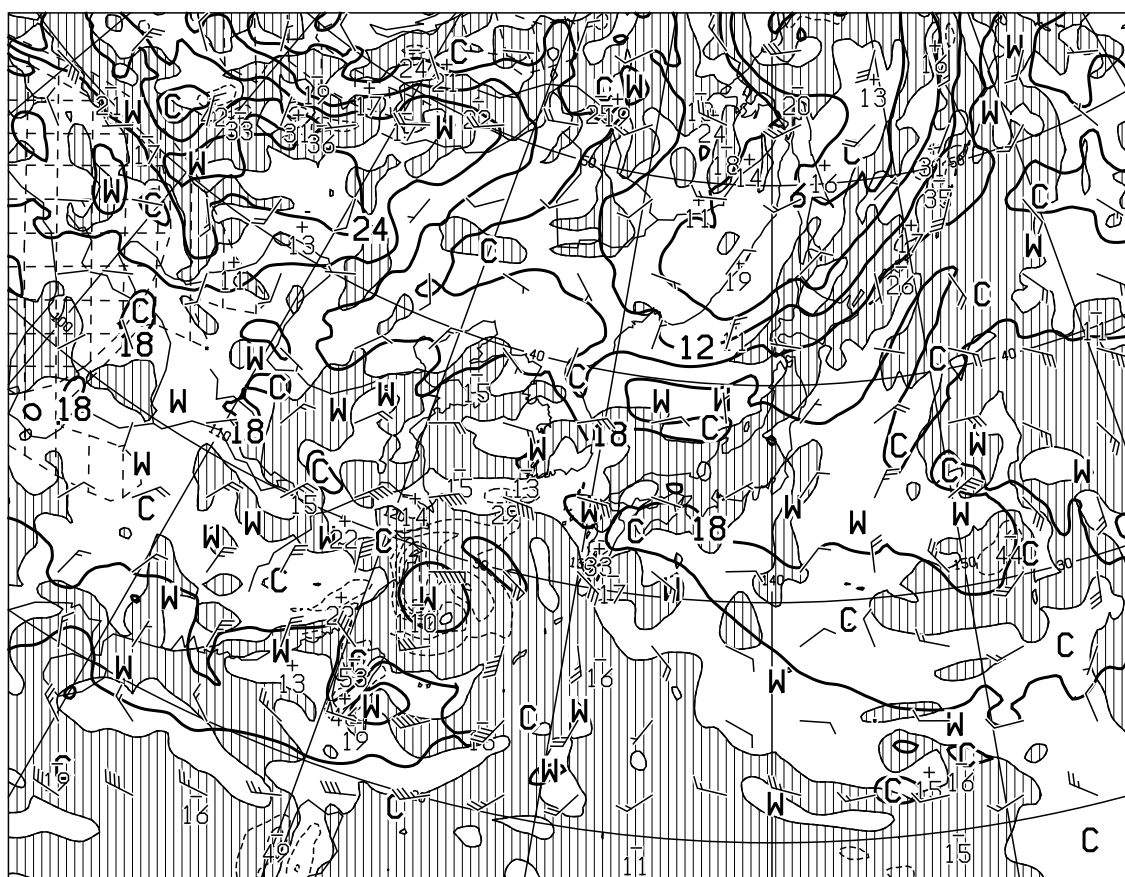
T=12 VALID 090000UTC TEMP (C), WIND ARROW AT 850hPa P-VEL (hPa/H) AT 700hPa
