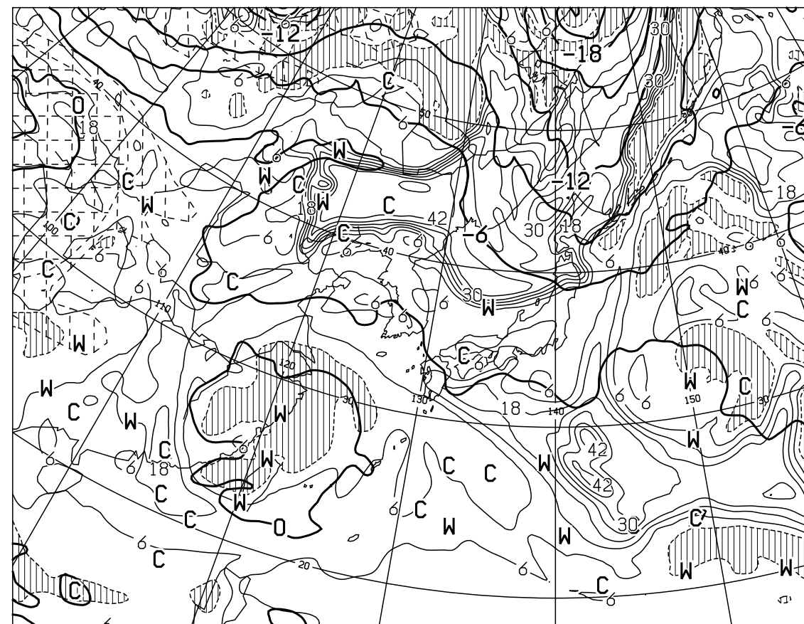
T=24 VALID 091200UTC TEMP (C) AT 500hPa T-TD (C) AT 700hPa
