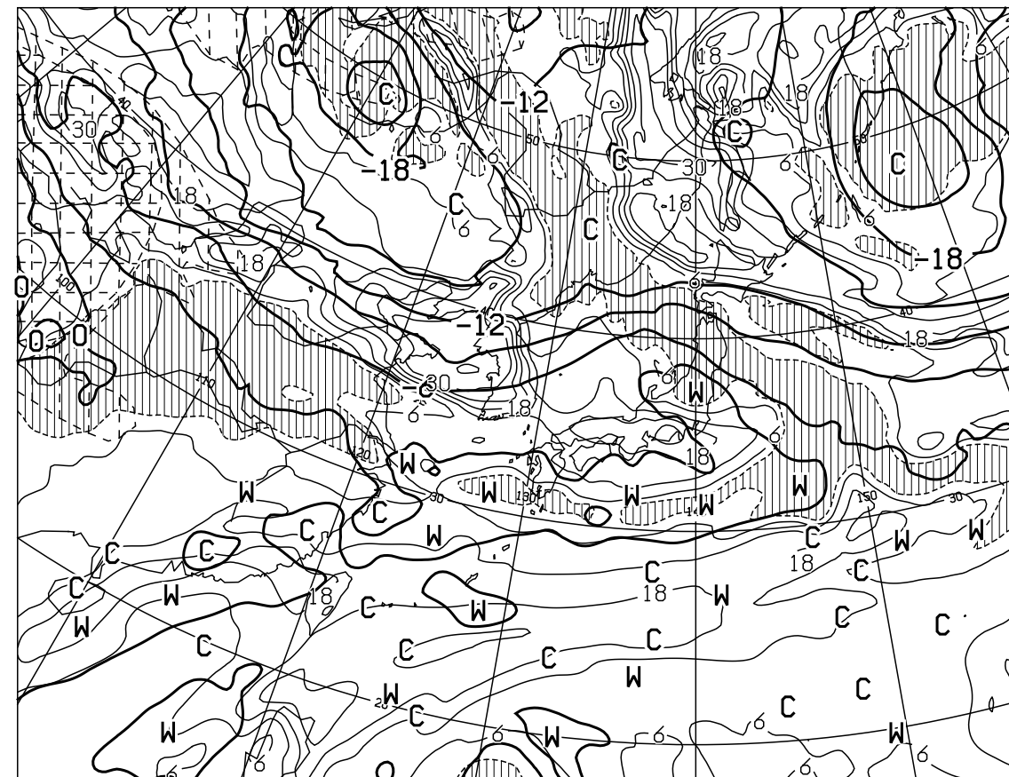
T=24 VALID 211200UTC TEMP (C) AT 500hPa T-TD (C) AT 700hPa
