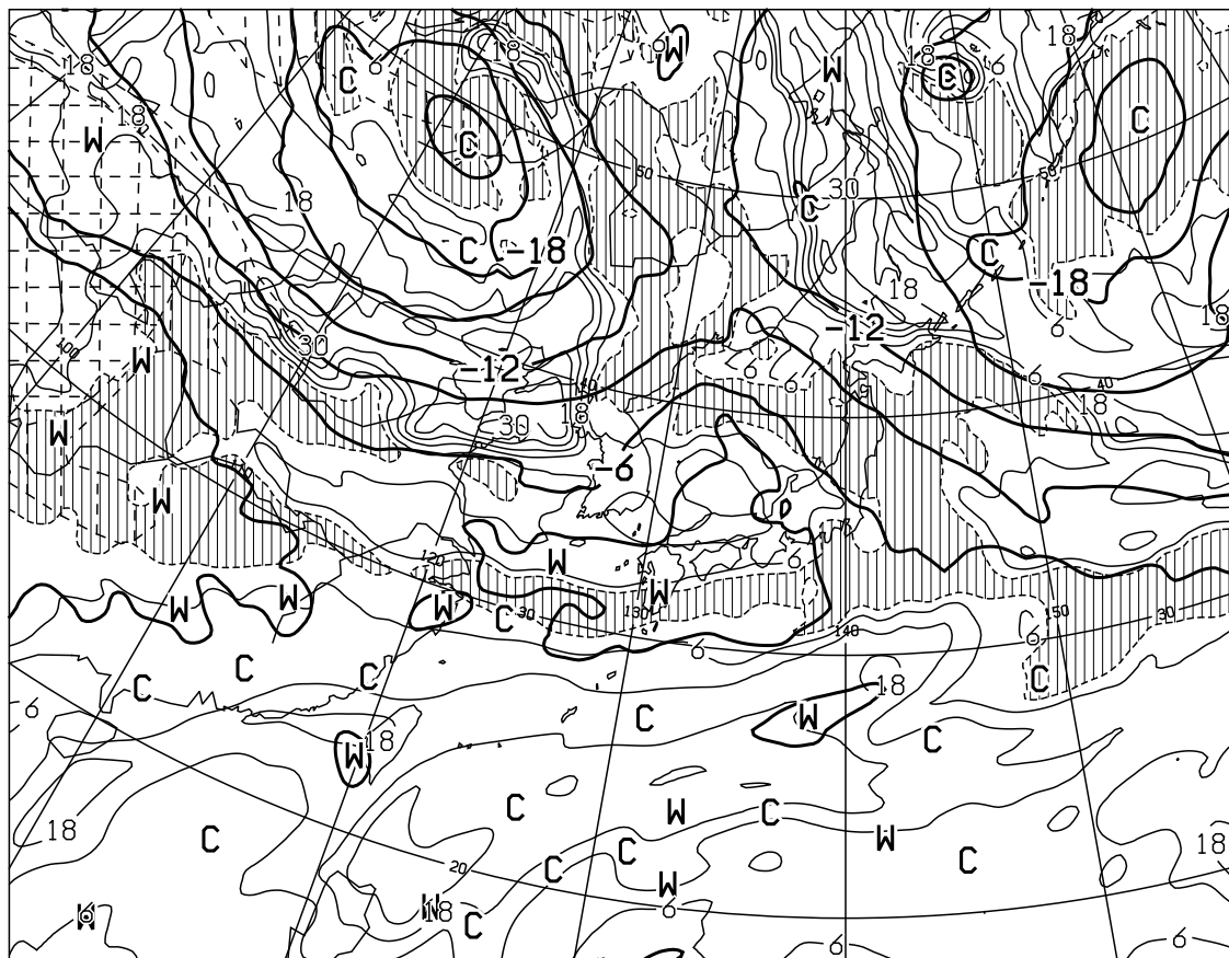
T=12 VALID 210000UTC TEMP (C) AT 500hPa T-TD (C) AT 700hPa
