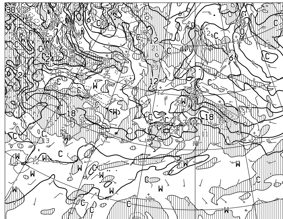
T=24 VALID 211200UTC TEMP (C), WIND ARROW AT 850hPa P-VEL (hPa/h) AT 700hPa
