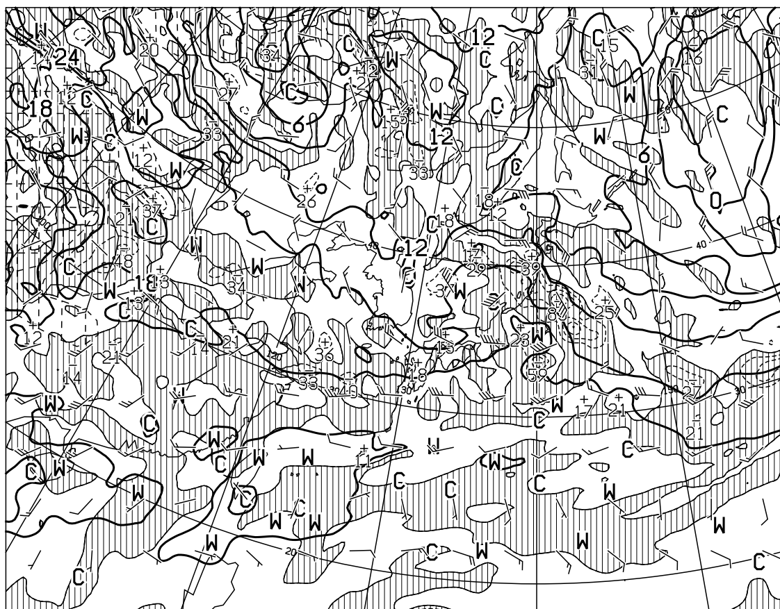
T=12 VALID 210000UTC TEMP (C), WIND ARROW AT 850hPa P-VEL (hPa/h) AT 700hPa
