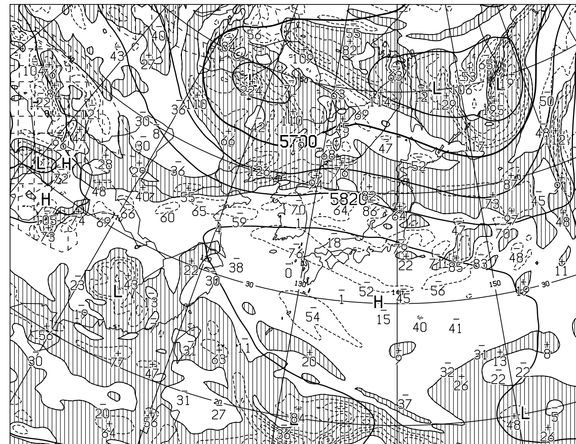
T=24 VALID 291200UTC HEIGHT(M),VORT(10**x-6/SEC) AT 500hPa
