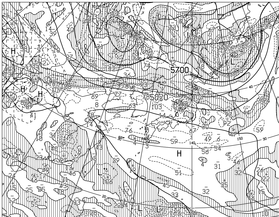
T=12 VALID 290000UTC HEIGHT(M),VORT(10**x-6/SEC) AT 500hPa
