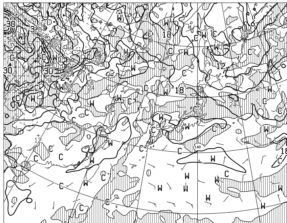
T=24 VALID 221200UTC TEMP (C), WIND ARROW AT 850hPa P-VEL (hPa/h) AT 700hPa
