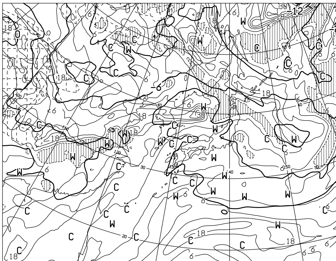
T=12 VALID 220000UTC TEMP (C) AT 500hPa T-TD (C) AT 700hPa
