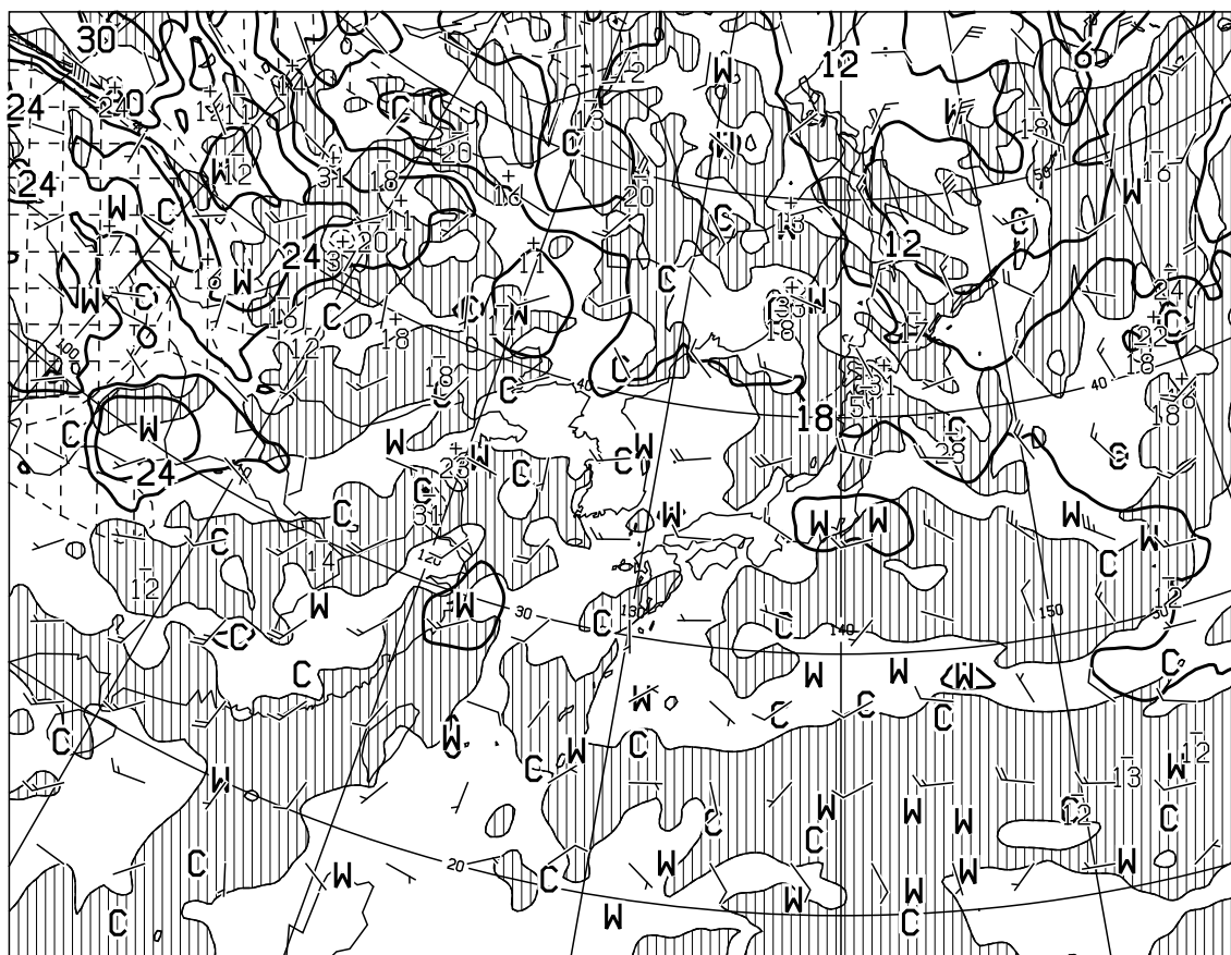
T=12 VALID 220000UTC TEMP (C), WIND ARROW AT 850hPa P-VEL (hPa/h) AT 700hPa
