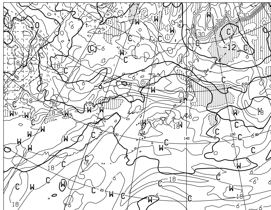
T=24 VALID 221200UTC TEMP (C) AT 500hPa T-TD (C) AT 700hPa
