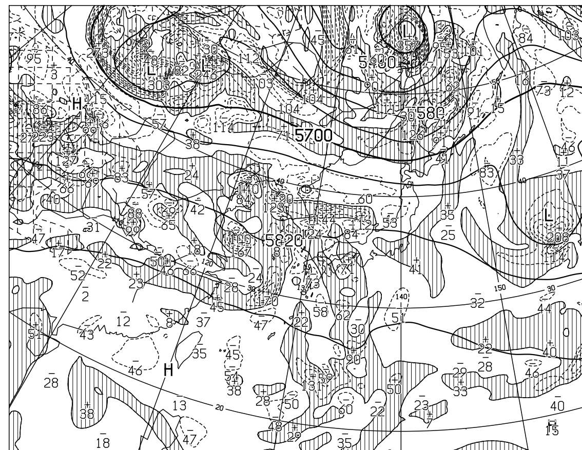
T=24 VALID 261200UTC HEIGHT(M),VORT(10××-6/SEC) AT 500hPa
