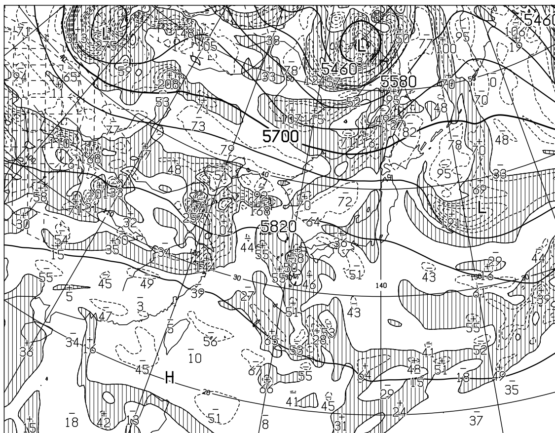
T=12 VALID 260000UTC HEIGHT(M),VORT(10××-6/SEC) AT 500hPa
