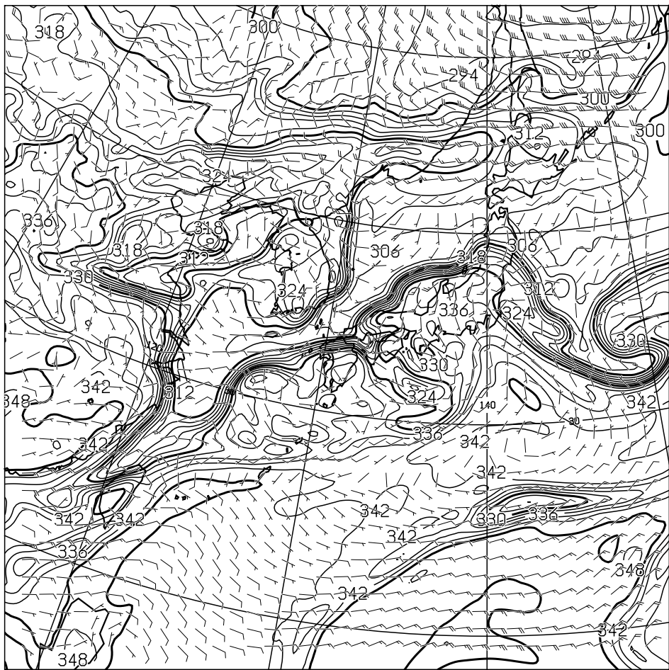
T=48 850hPa: E.P.TEMP(K),WIND(KNOTS) VALID 231200UTC
