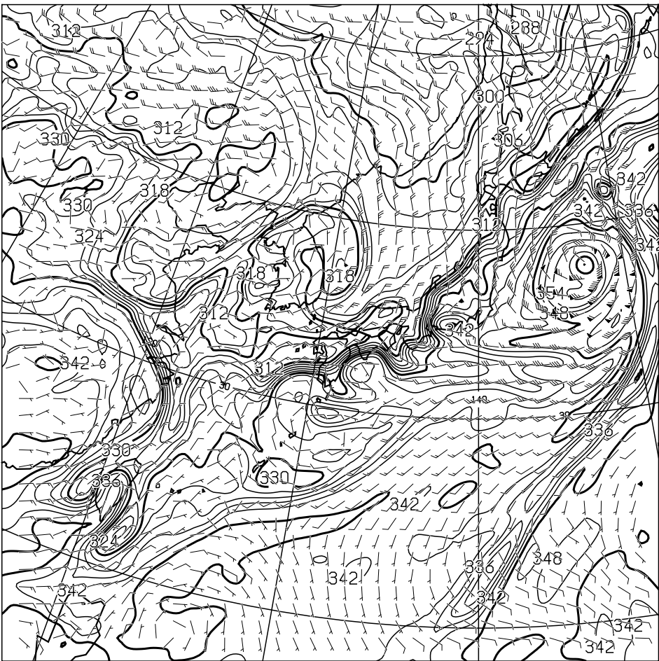
T=12 850hPa: E.P.TEMP(K),WIND(KNOTS) VALID 220000UTC
