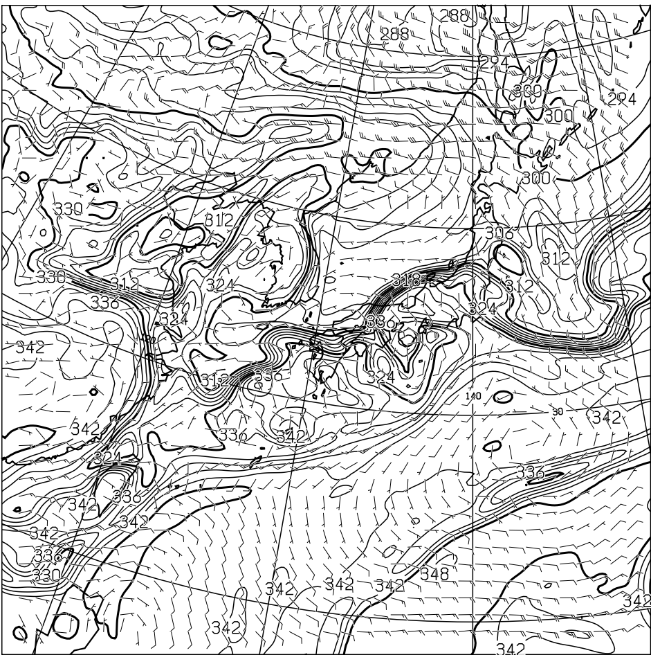
T=36 850hPa: E.P.TEMP(K),WIND(KNOTS) VALID 230000UTC
