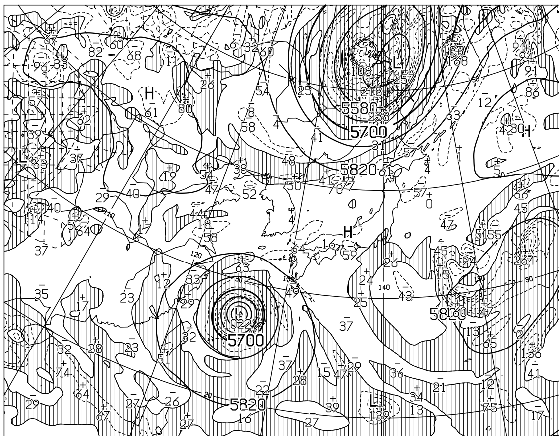
T=12 VALID 080000UTC HEIGHT(M),VORT(10**+6/SEC) AT 500hPa
