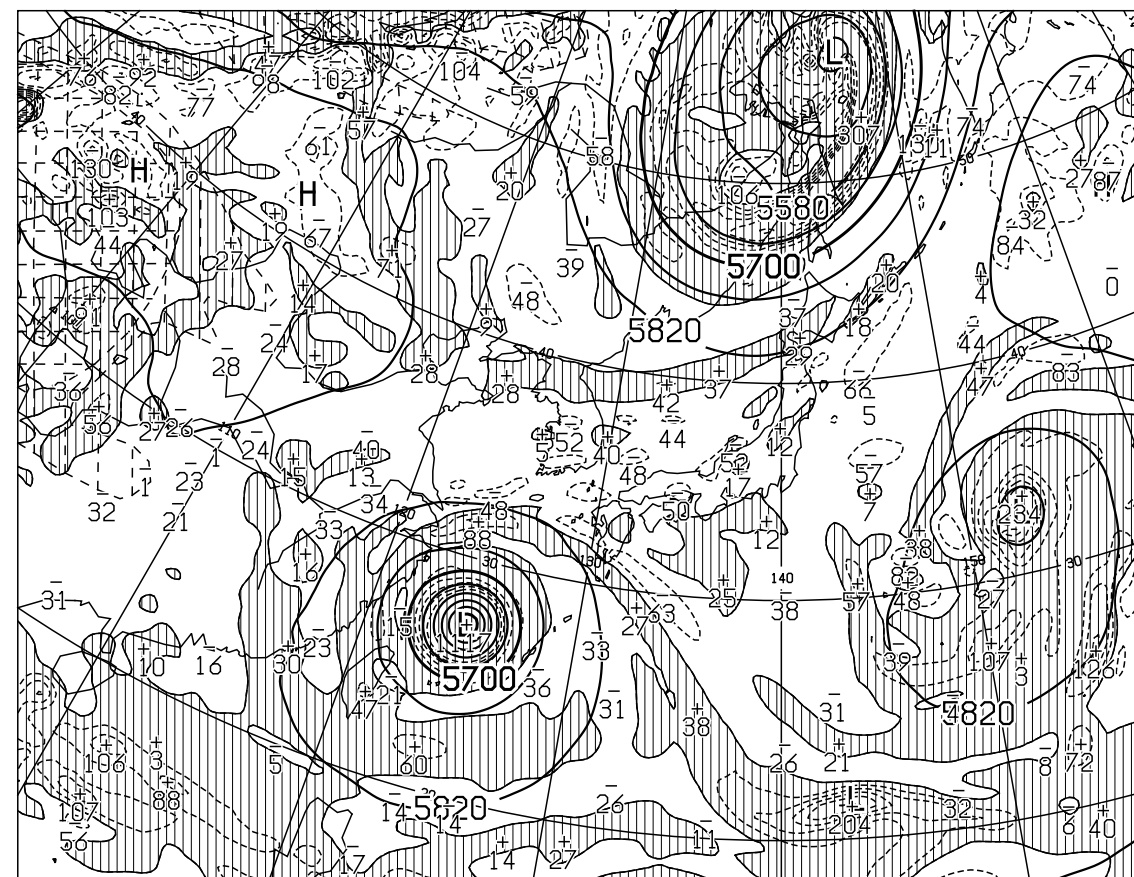
T=24 VALID 081200UTC HEIGHT(M),VORT(10**+6/SEC) AT 500hPa
