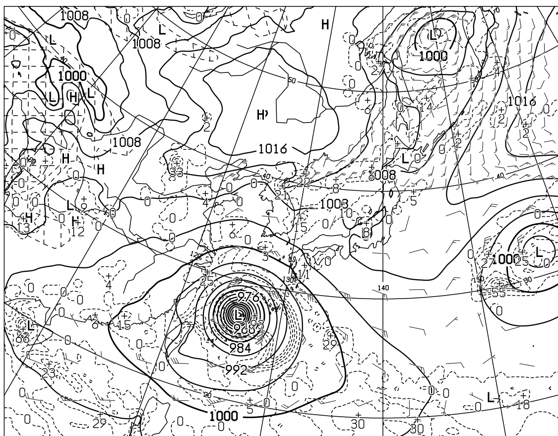
T=12 VALID 080000UTC SURFACE PRESS(hPa),PRECIP(MM) (00-12) WIND ARROW AT SURFACE
