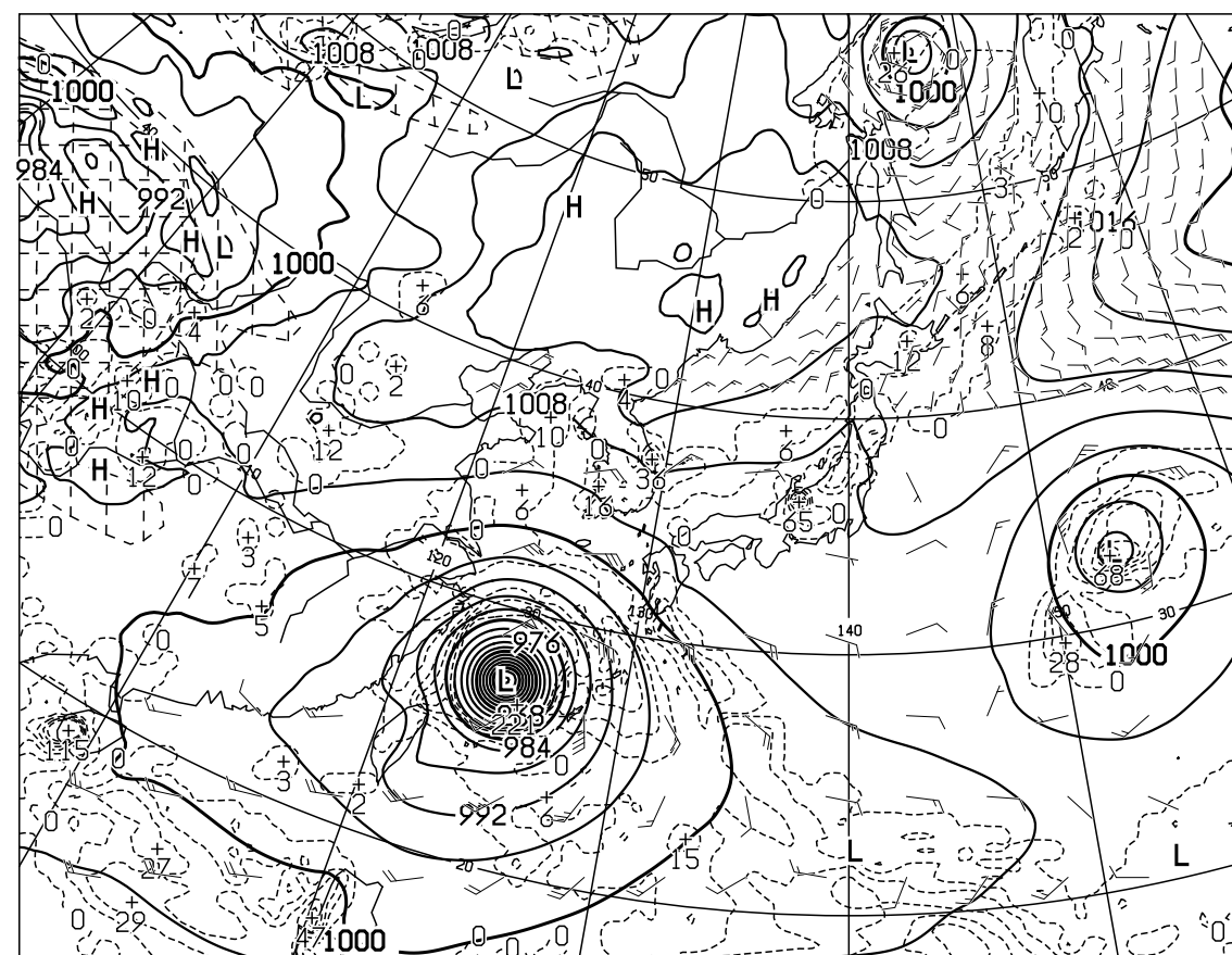
T=24 VALID 081200UTC SURFACE PRESS(hPa),PRECIP(MM) (12-24) WIND ARROW AT SURFACE
