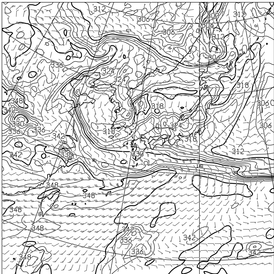
T=48 850hPa: E.P.TEMP(K),WIND(KNOTS) VALID 141200UTC
