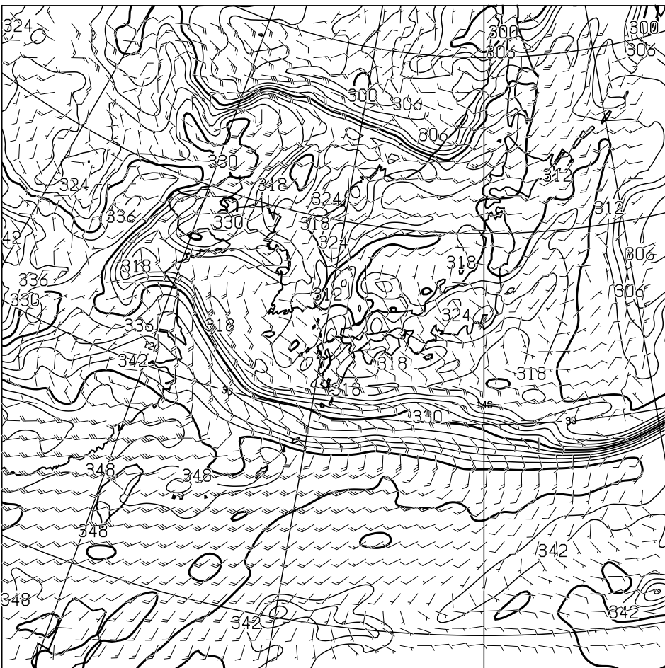
T=36 850hPa: E.P.TEMP(K),WIND(KNOTS) VALID 140000UTC
