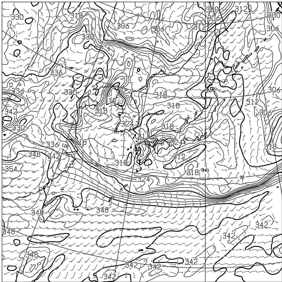
T=24 850hPa: E.P.TEMP(K),WIND(KNOTS) VALID 131200UTC
