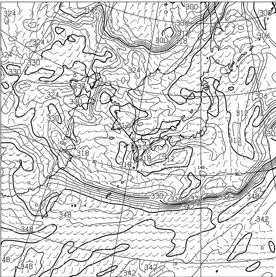
T=12 850hPa: E.P.TEMP(K),WIND(KNOTS) VALID 130000UTC
