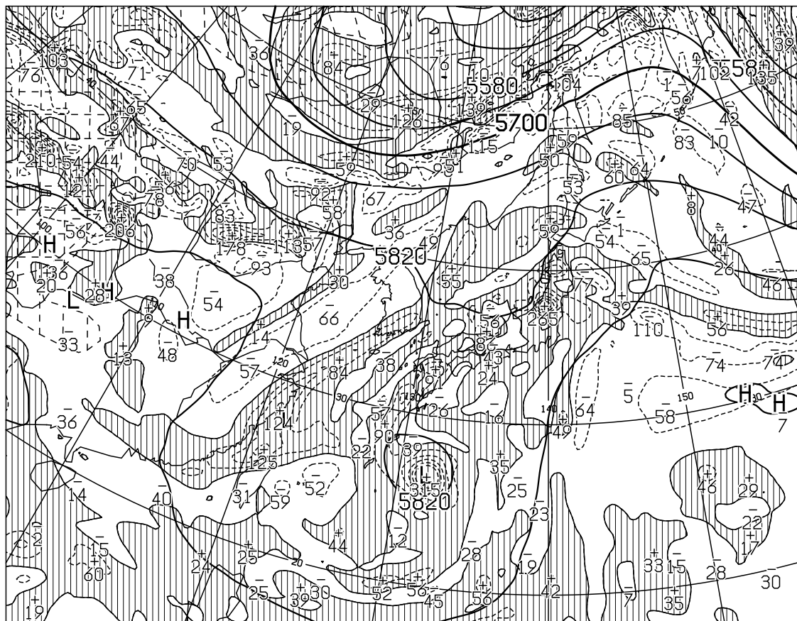
T=12 VALID 070000UTC HEIGHT(M),VORT(10 -6 /SEC) AT 500hPa
