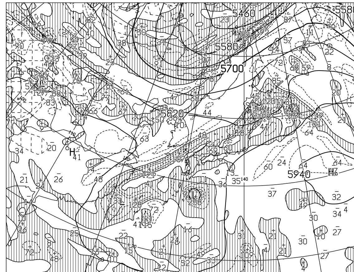
T=24 VALID 071200UTC HEIGHT(M),VORT(10 -6 /SEC) AT 500hPa
