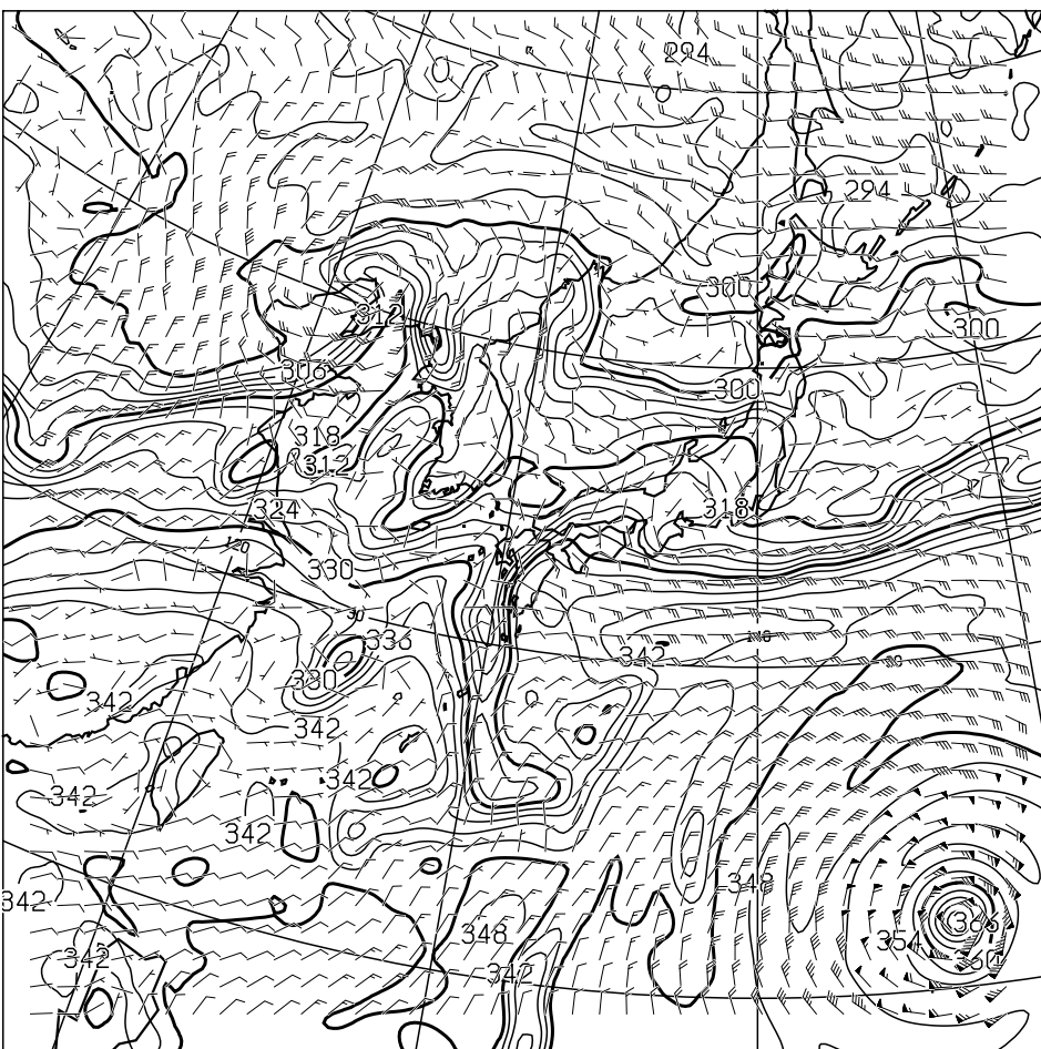
T=36 850hPa: E.P.TEMP(K),WIND(KNOTS) VALID 040000UTC
