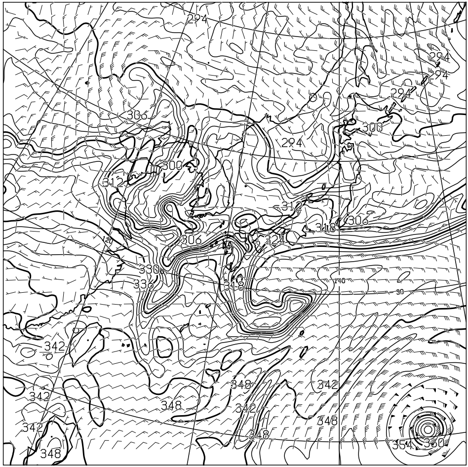
T=24 850hPa: E.P.TEMP(K),WIND(KNOTS) VALID 031200UTC
