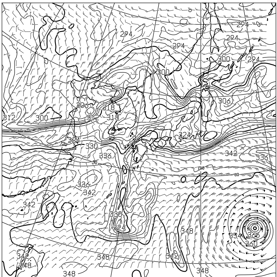
T=48 850hPa: E.P.TEMP(K),WIND(KNOTS) VALID 041200UTC
