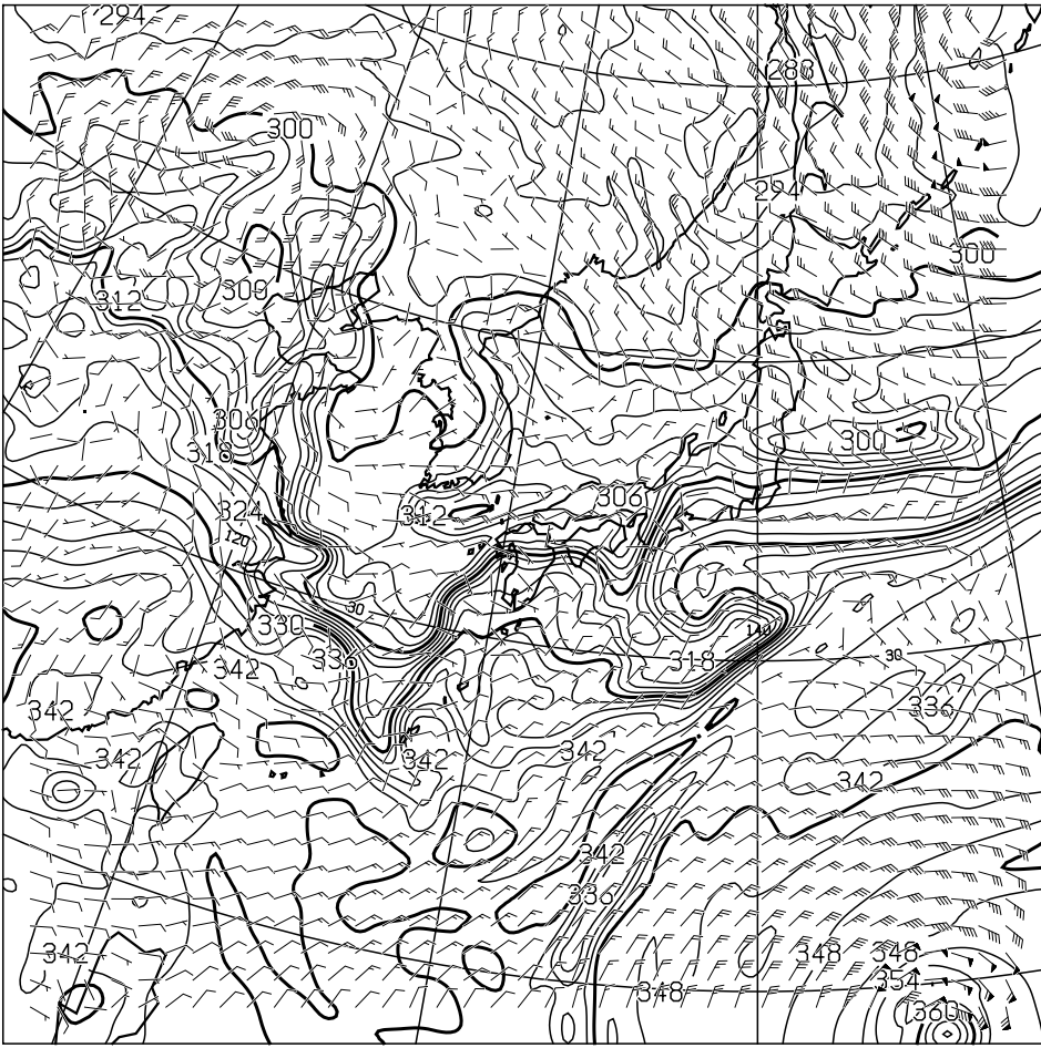
T=12 850hPa: E.P.TEMP(K),WIND(KNOTS) VALID 030000UTC
