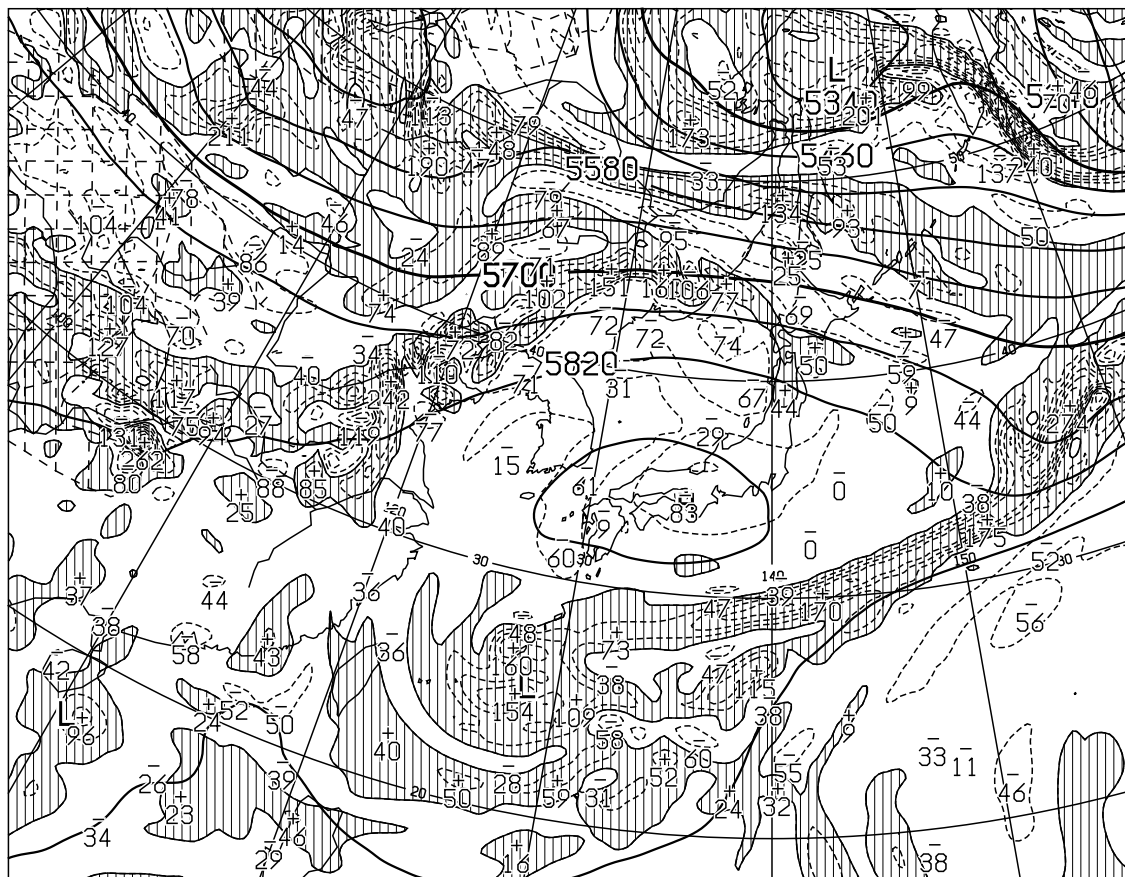
T=12 VALID 180000UTC HEIGHT (M), VORT (10 \times -6/SEC) AT 500hPa
