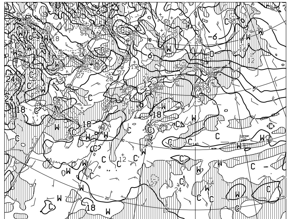
T=24 VALID 181200UTC TEMP( C), WIND ARROW AT 850hPa P-VEL(hPa/H) AT 700hPa
