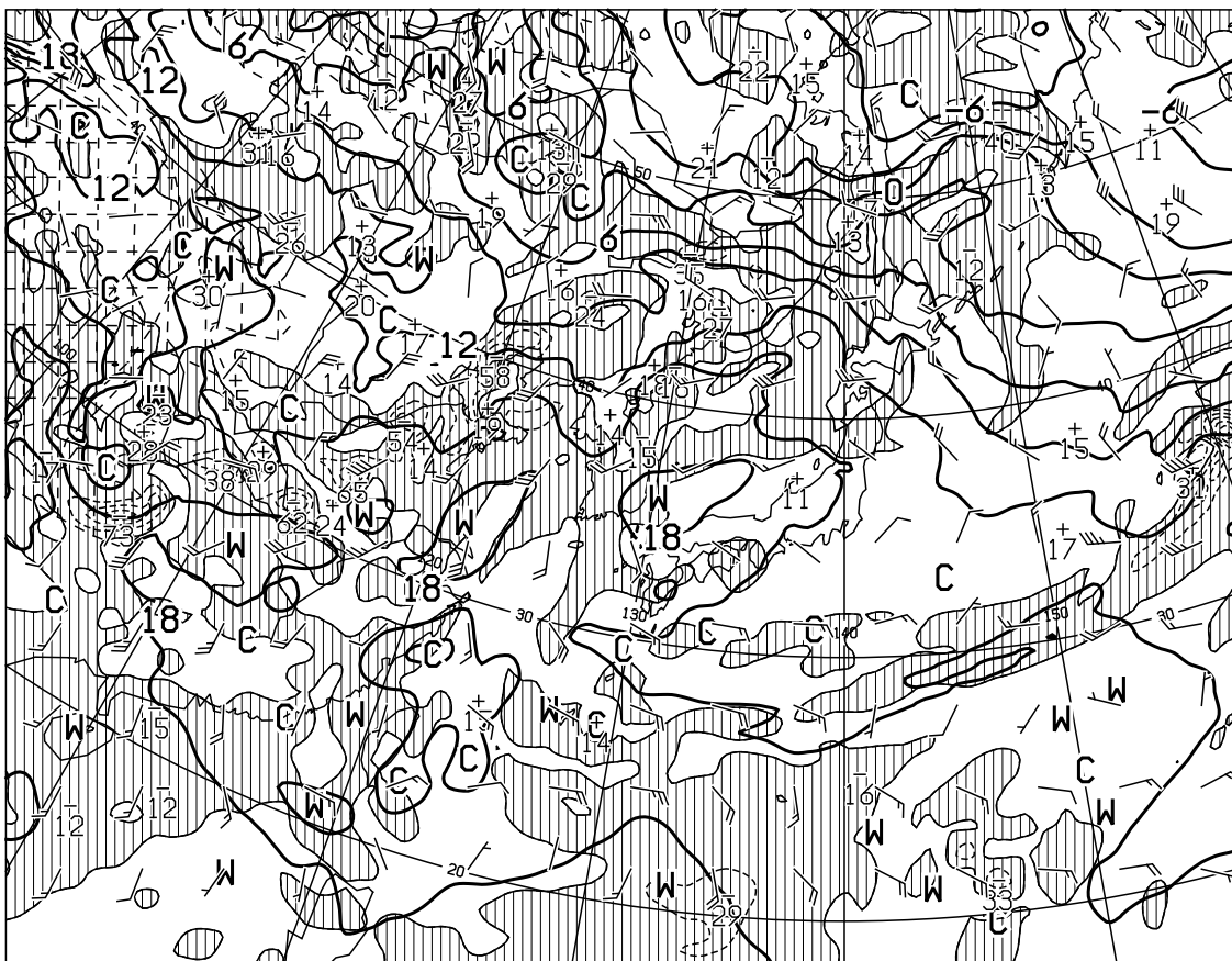
T=12 VALID 180000UTC TEMP( C), WIND ARROW AT 850hPa P-VEL(hPa/H) AT 700hPa
