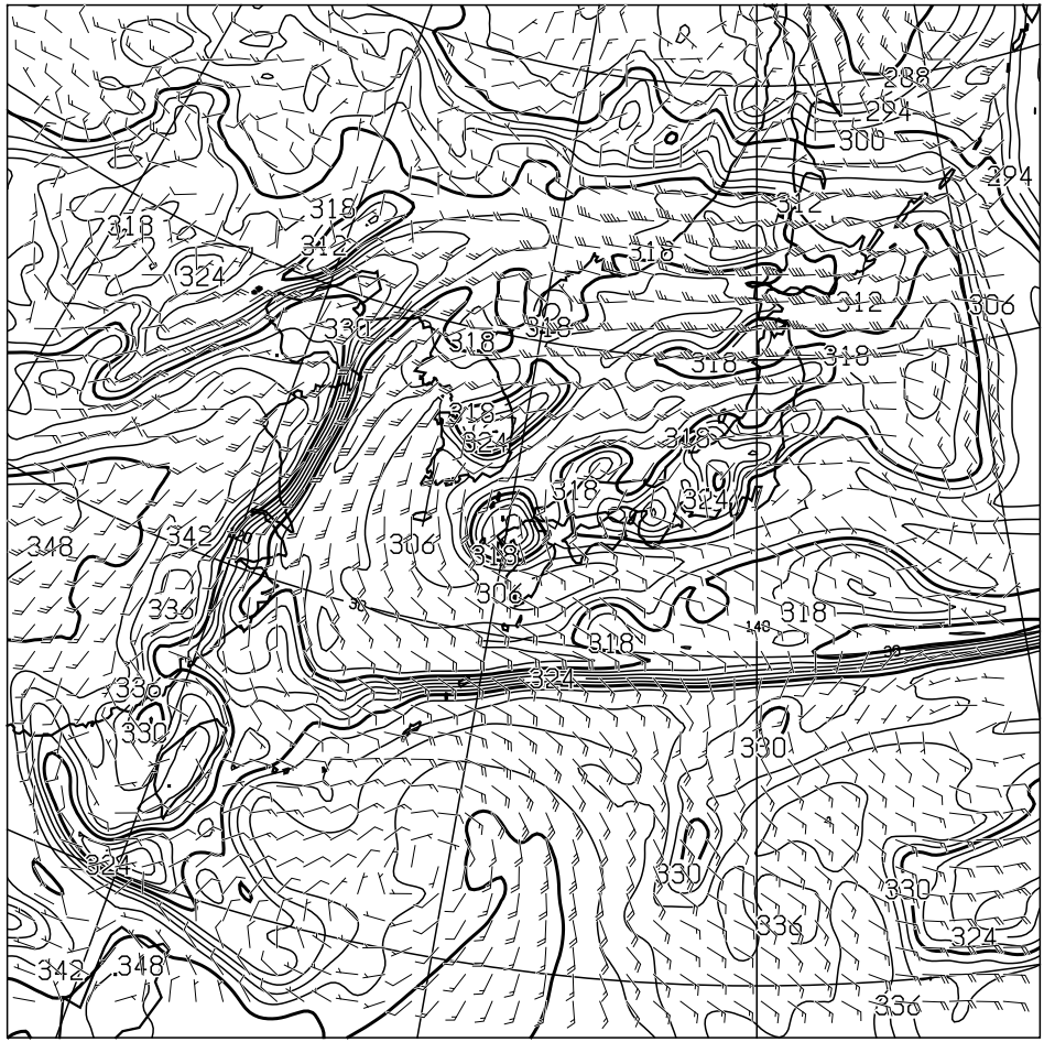
T=24 850hPa: E.P.TEMP(K),WIND(KNOTS) VALID 181200UTC
