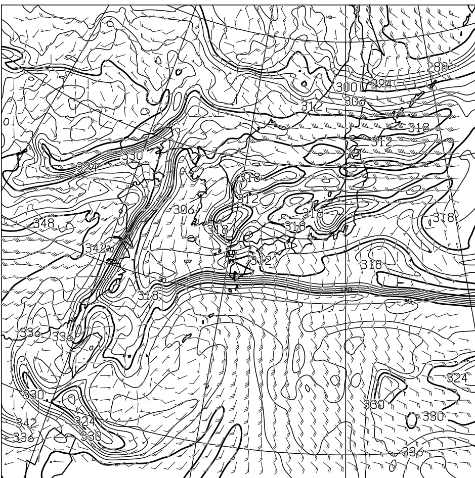
T=36 850hPa: E.P.TEMP(K),WIND(KNOTS) VALID 190000UTC
