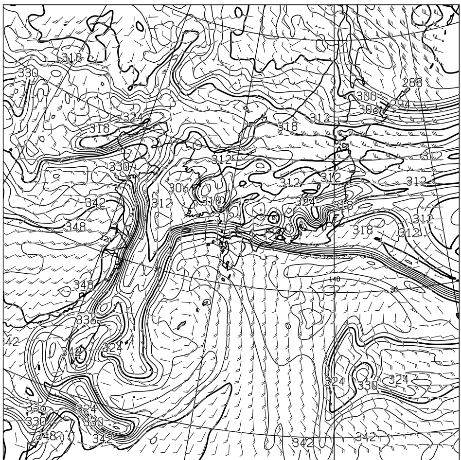
T=48 850hPa: E.P.TEMP(K),WIND(KNOTS) VALID 191200UTC
