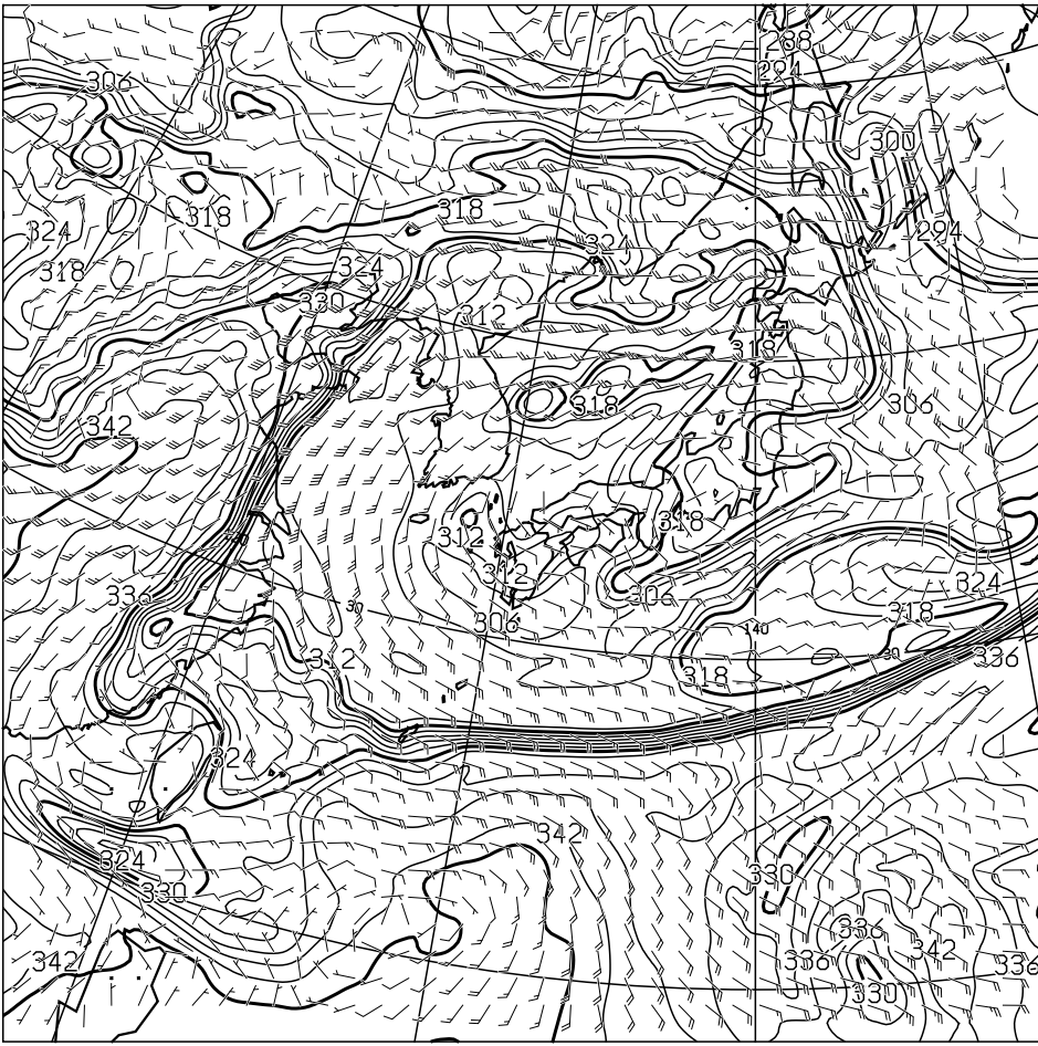
T=12 850hPa: E.P.TEMP(K),WIND(KNOTS) VALID 180000UTC
