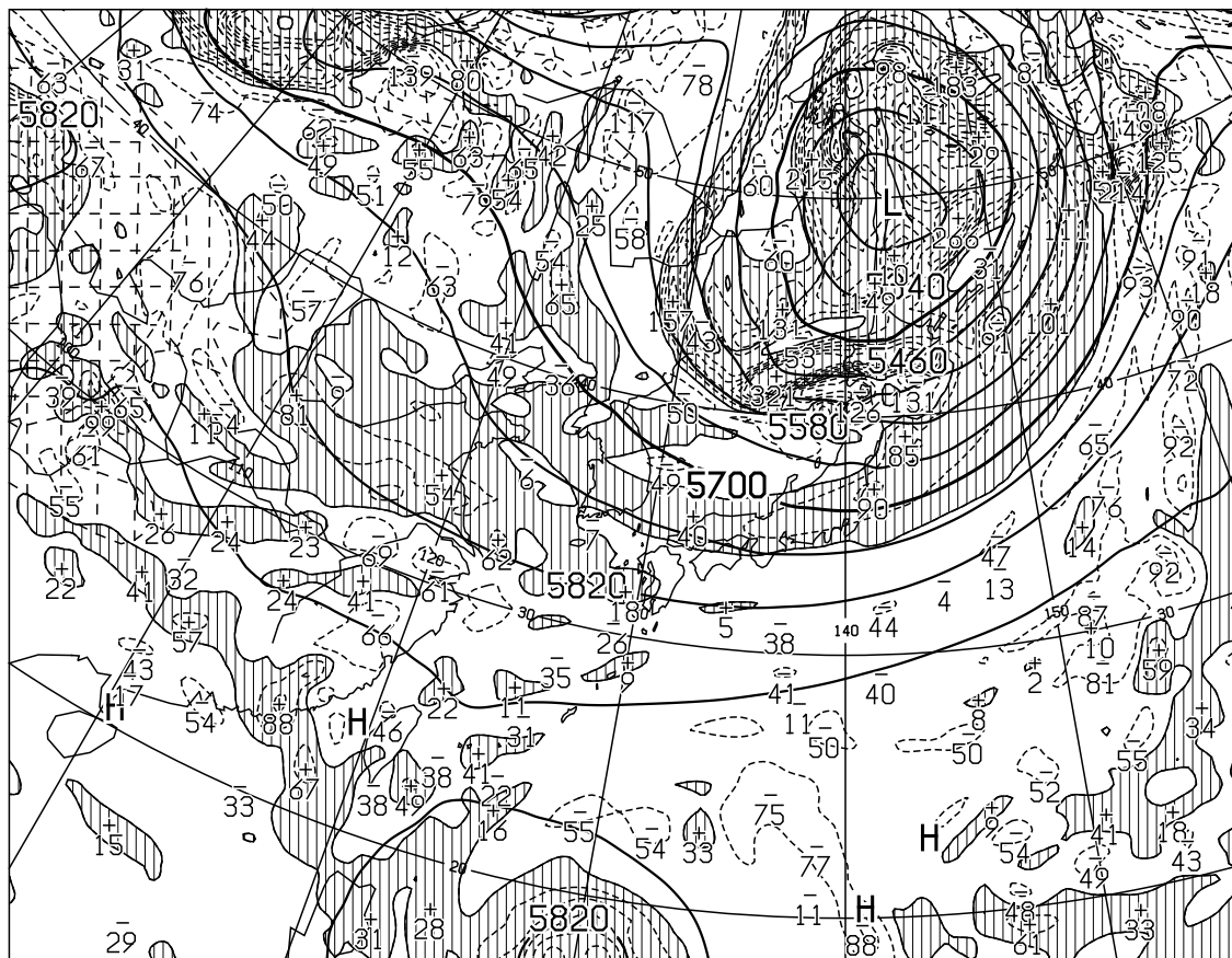
T=12 VALID 300000UTC HEIGHT(M),VORT(10**6/SEC) AT 500hPa
