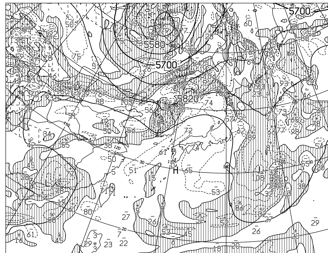
T=24 VALID 141200UTC HEIGHT(M),VORT(10 \times -6/SEC) AT 500hPa
