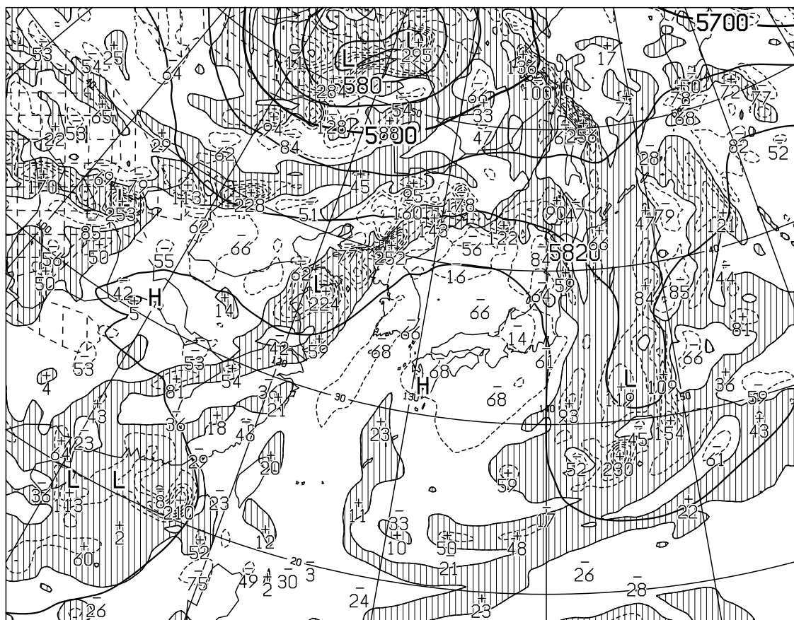
T=12 VALID 140000UTC HEIGHT(M),VORT(10 \times -6/SEC) AT 500hPa
