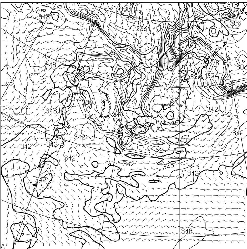
T=36 850hPa: E.P.TEMP(K),WIND(KNOTS) VALID 290000UTC
