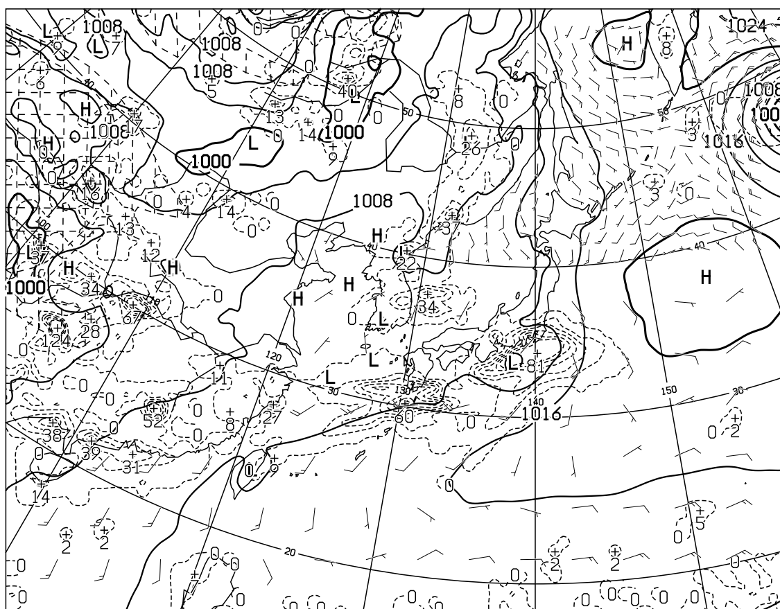
T=12 VALID 180000UTC SURFACE PRESS(hPa),PRECIP(MM) (00-12) WIND ARROW AT SURFACE
