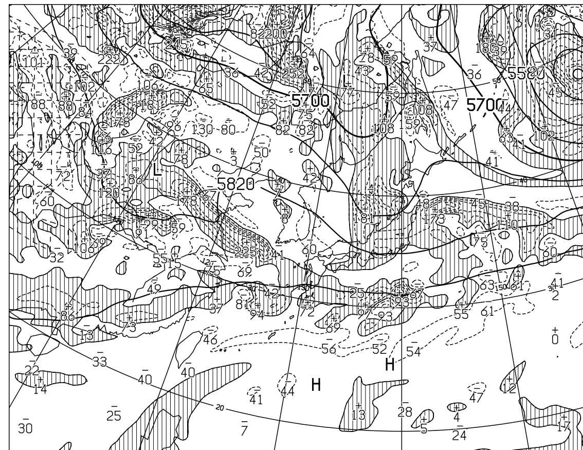
T=24 VALID 181200UTC HEIGHT(M),VORT(10**x-6/SEC) AT 500hPa
