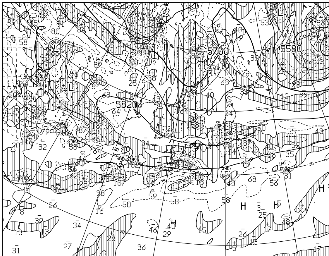
T=12 VALID 180000UTC HEIGHT(M),VORT(10**x-6/SEC) AT 500hPa
