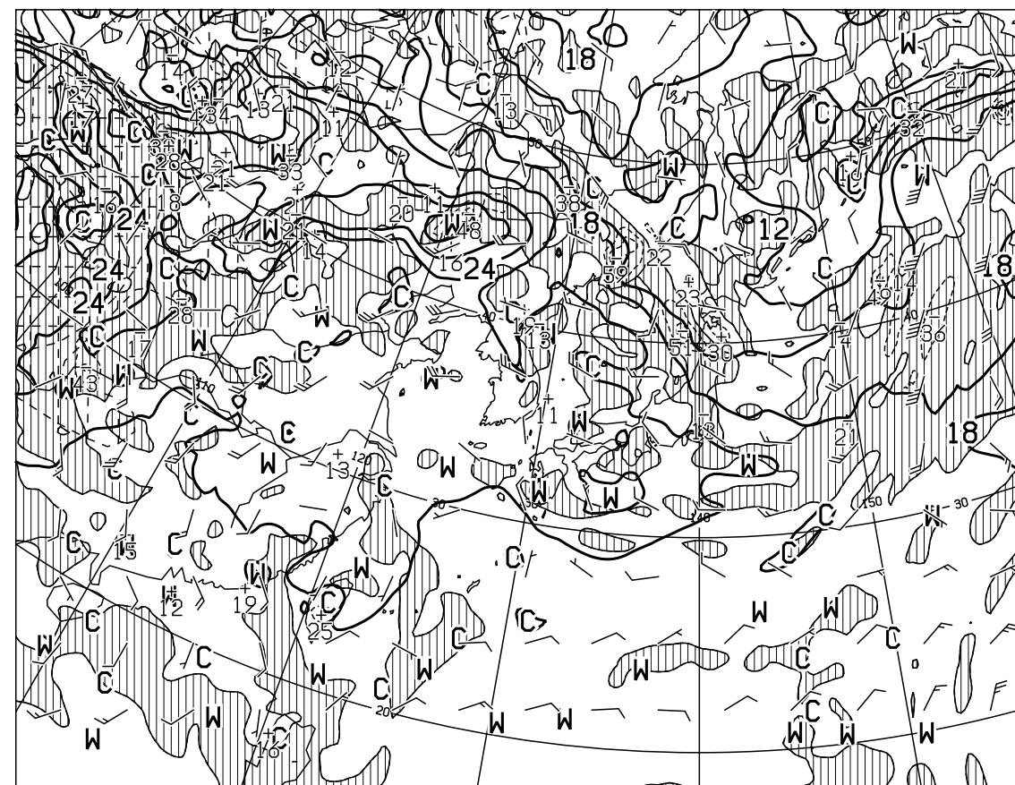
T=24 VALID 311200UTC TEMP ( C ), WIND ARROW AT 850hPa P-VEL (hPa/h) AT 700hPa
