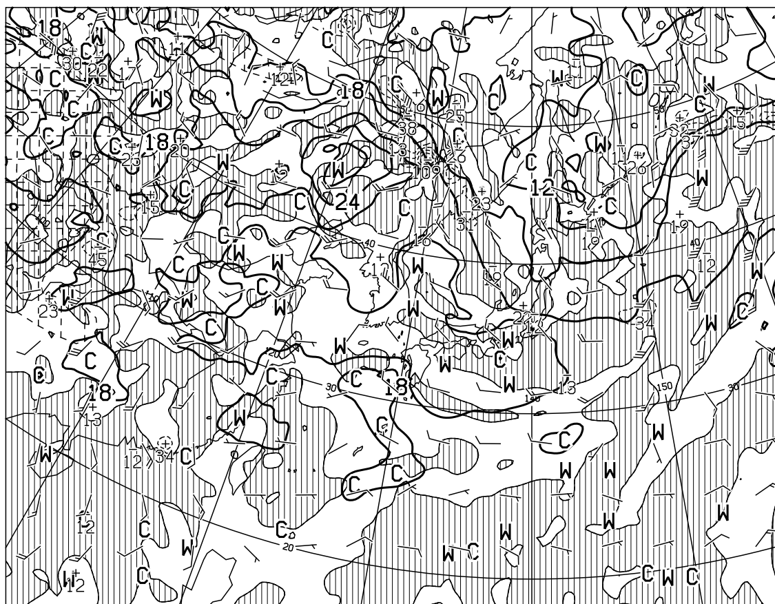
T=12 VALID 310000UTC TEMP ( C ), WIND ARROW AT 850hPa P-VEL (hPa/h) AT 700hPa
