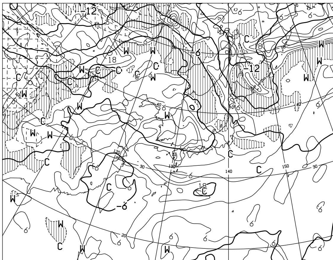
T=12 VALID 310000UTC TEMP ( C ) AT 500hPa T-TD ( C ) AT 700hPa
