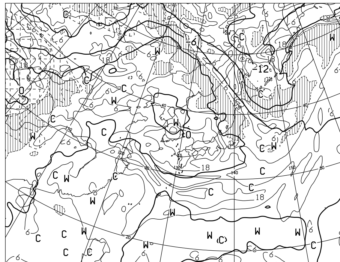
T=24 VALID 311200UTC TEMP ( C ) AT 500hPa T-TD ( C ) AT 700hPa
