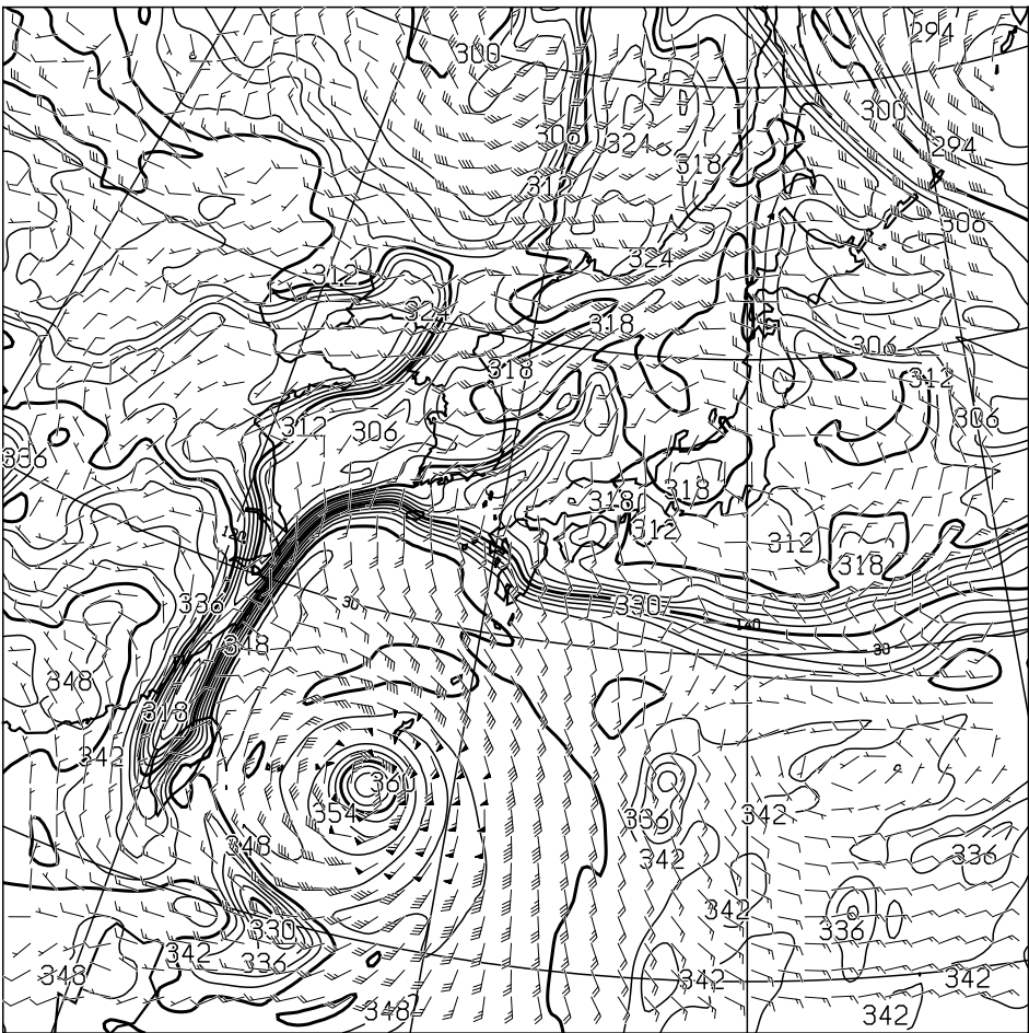
T=12 850hPa: E.P.TEMP(K),WIND(KNOTS) VALID 010000UTC
