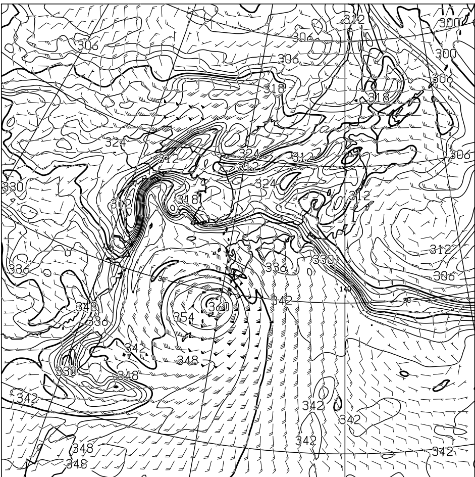
T=36 850hPa: E.P.TEMP(K),WIND(KNOTS) VALID 020000UTC
