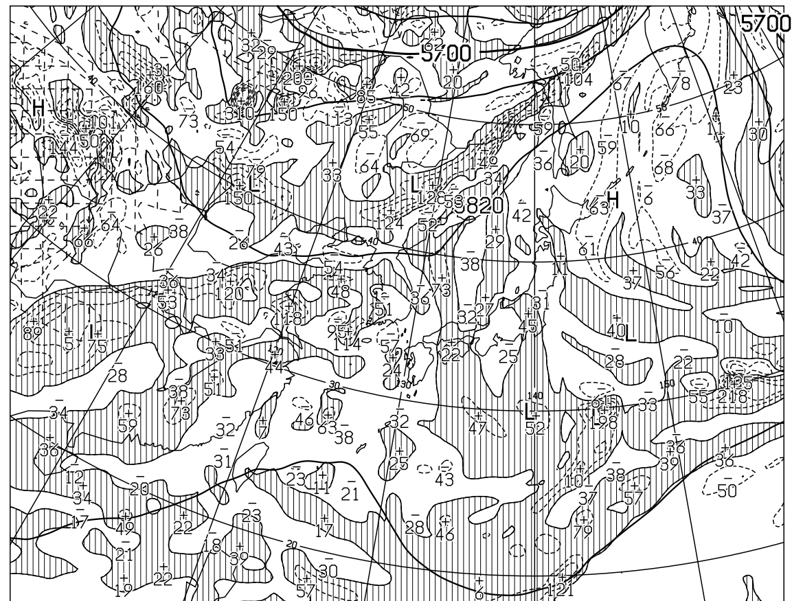
T=24 VALID 141200UTC HEIGHT(M),VORT(10 \times -6/SEC) AT 500hPa
