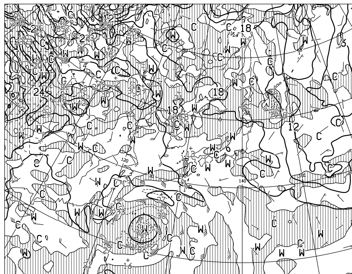
T=24 VALID 101200UTC TEMP (C), WIND ARROW AT 850hPa P-VEL (hPa/h) AT 700hPa
