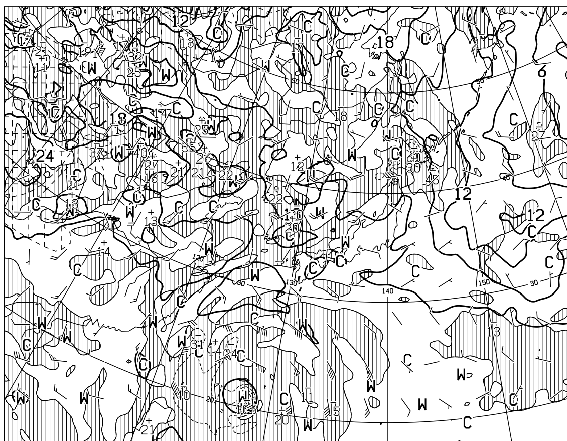
T=12 VALID 100000UTC TEMP (C), WIND ARROW AT 850hPa P-VEL (hPa/h) AT 700hPa
