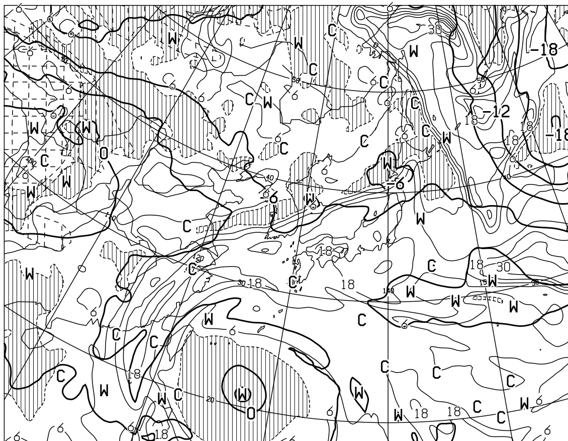
T=12 VALID 100000UTC TEMP (C) AT 500hPa T-TD (C) AT 700hPa
