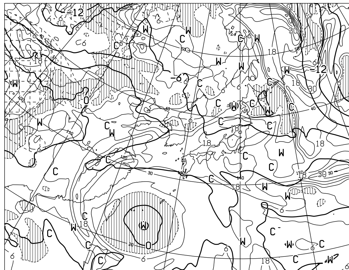
T=24 VALID 101200UTC TEMP (C) AT 500hPa T-TD (C) AT 700hPa
