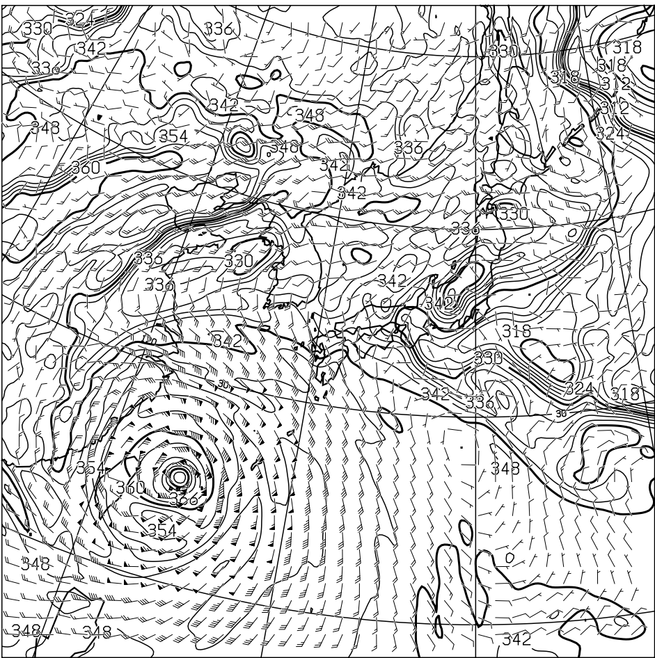
T=36 850hPa: E.P.TEMP(K),WIND(KNOTS) VALID 110000UTC
