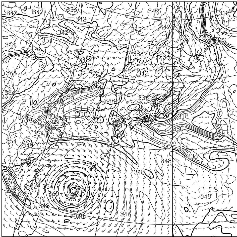
T=24 850hPa: E.P.TEMP(K),WIND(KNOTS) VALID 101200UTC
