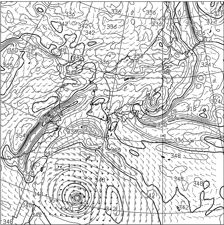
T=12 850hPa: E.P.TEMP(K),WIND(KNOTS) VALID 100000UTC
