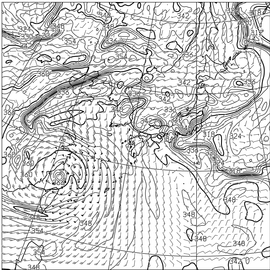
T=48 850hPa: E.P.TEMP(K),WIND(KNOTS) VALID 111200UTC
