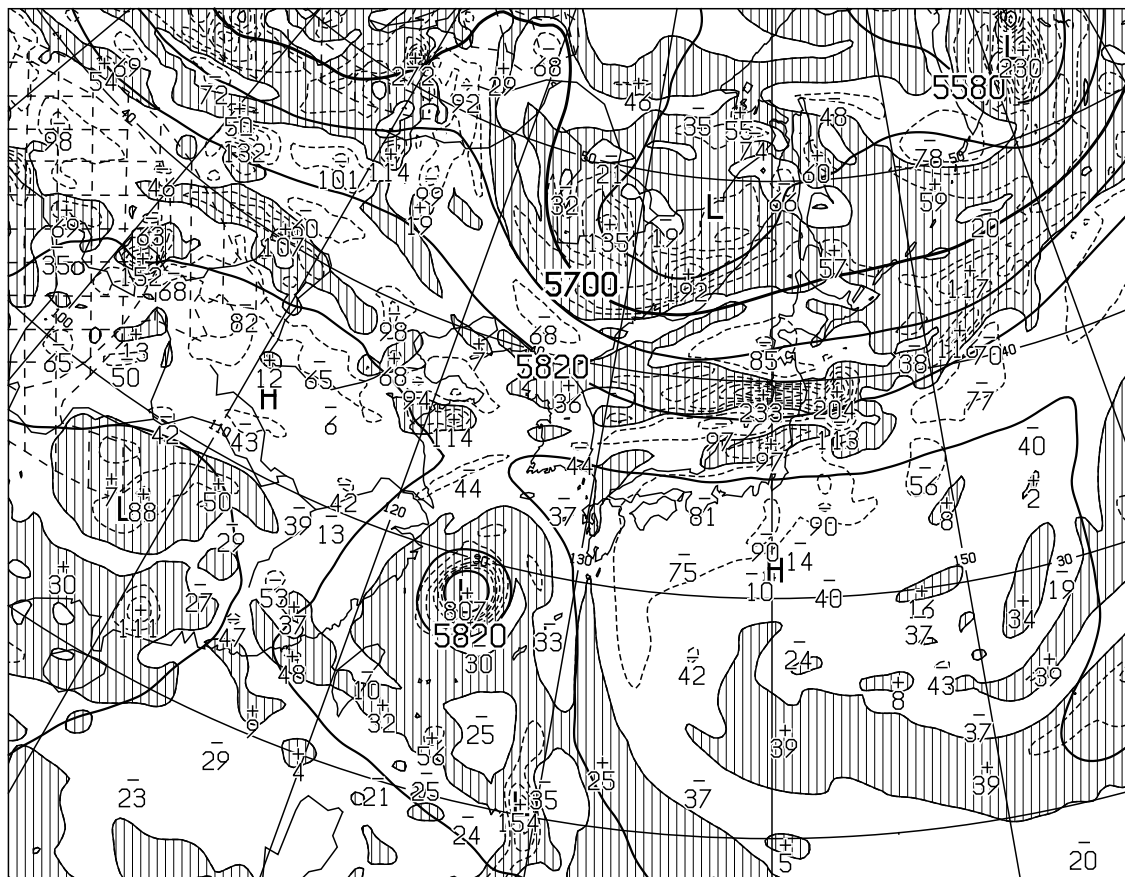
T=12 VALID 270000UTC HEIGHT(M),VORT(10 -6 /SEC) AT 500hPa
