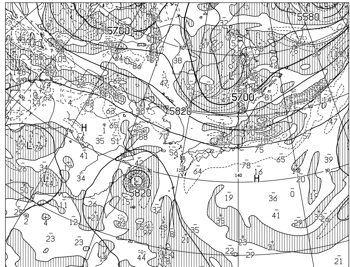
T=24 VALID 271200UTC HEIGHT(M),VORT(10 -6 /SEC) AT 500hPa
