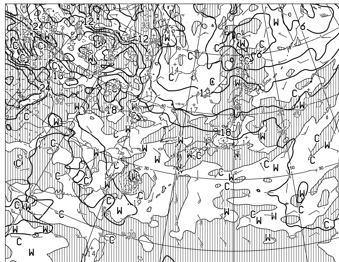
T=24 VALID 271200UTC TEMP (C), WIND ARROW AT 850hPa P-VEL (hPa/H) AT 700hPa
