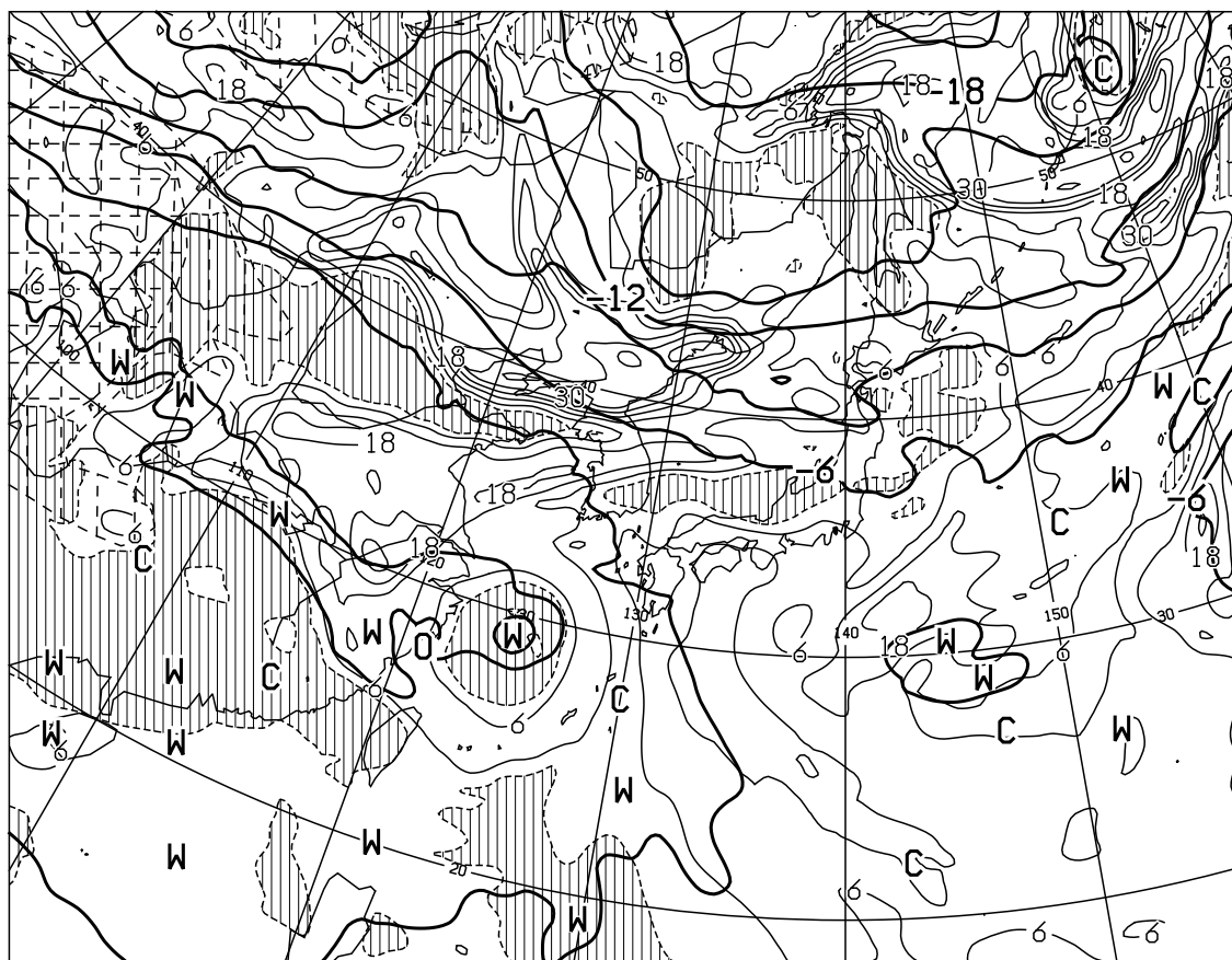
T=12 VALID 270000UTC TEMP (C) AT 500hPa T-TD (C) AT 700hPa
