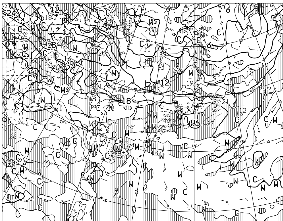
T=12 VALID 270000UTC TEMP (C), WIND ARROW AT 850hPa P-VEL (hPa/H) AT 700hPa
