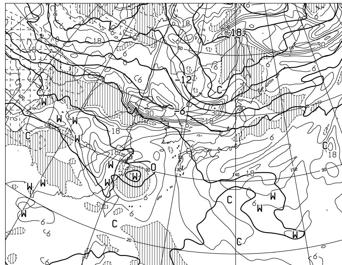
T=24 VALID 271200UTC TEMP (C) AT 500hPa T-TD (C) AT 700hPa
