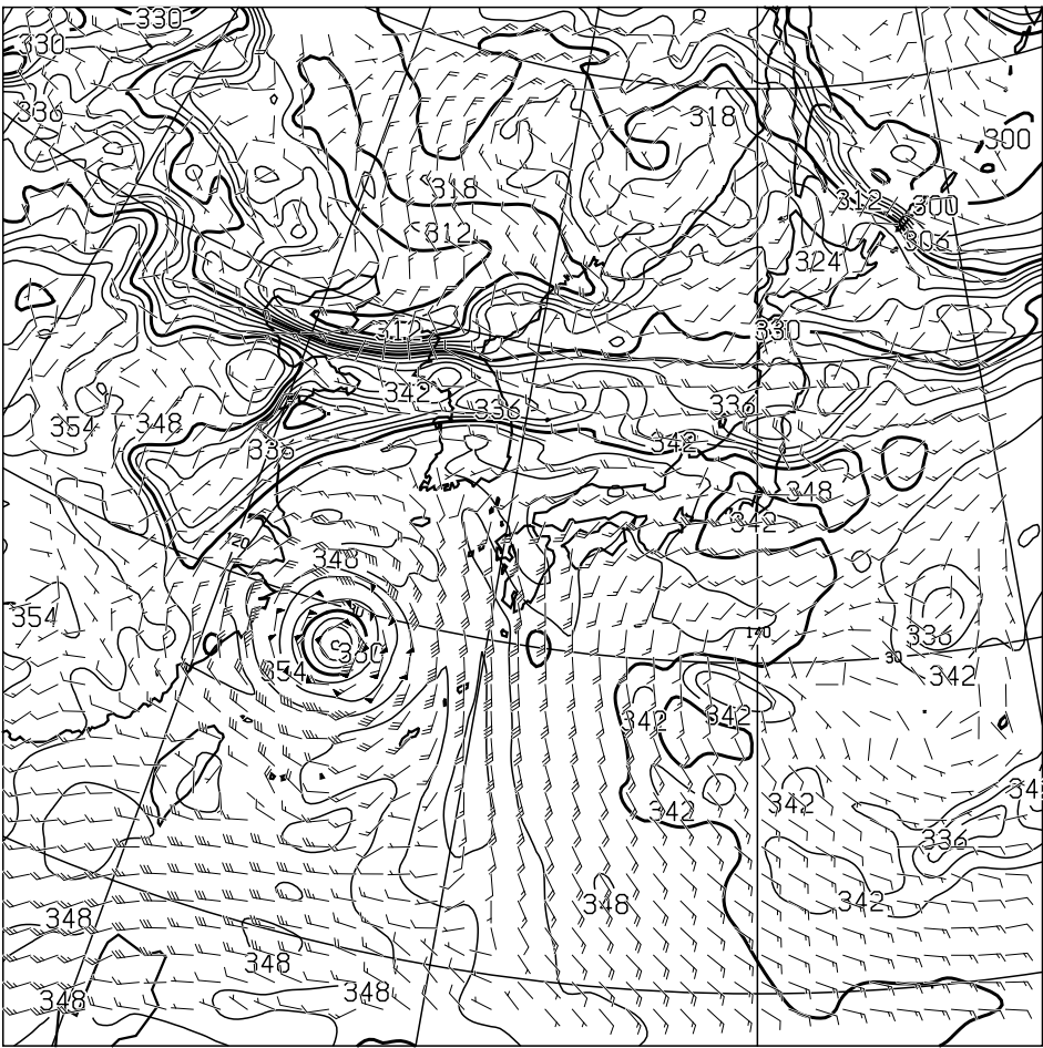
T=12 850hPa: E.P.TEMP(K),WIND(KNOTS) VALID 270000UTC
