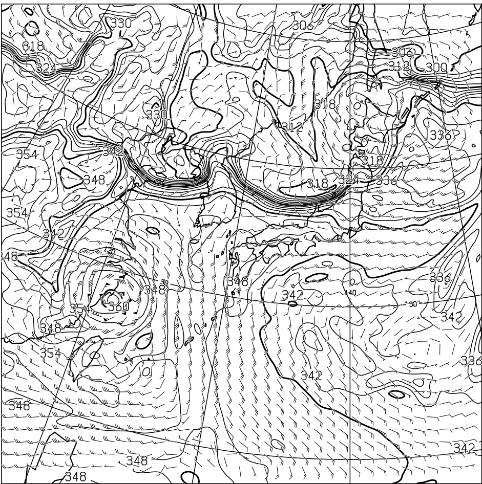
T=36 850hPa: E.P.TEMP(K),WIND(KNOTS) VALID 280000UTC
