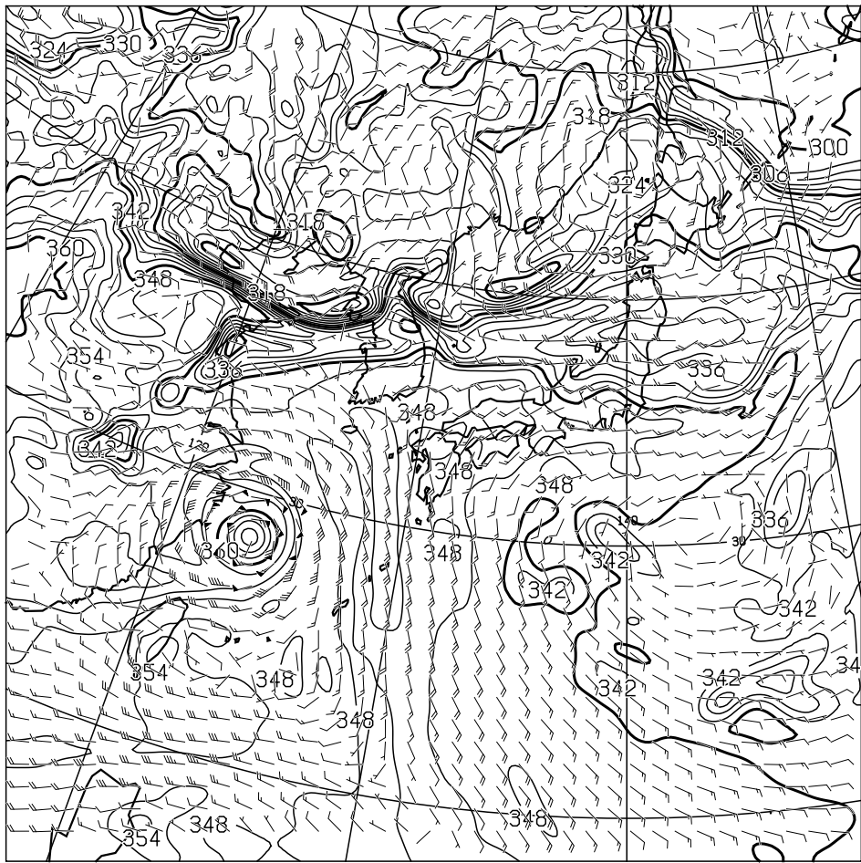
T=24 850hPa: E.P.TEMP(K),WIND(KNOTS) VALID 271200UTC
