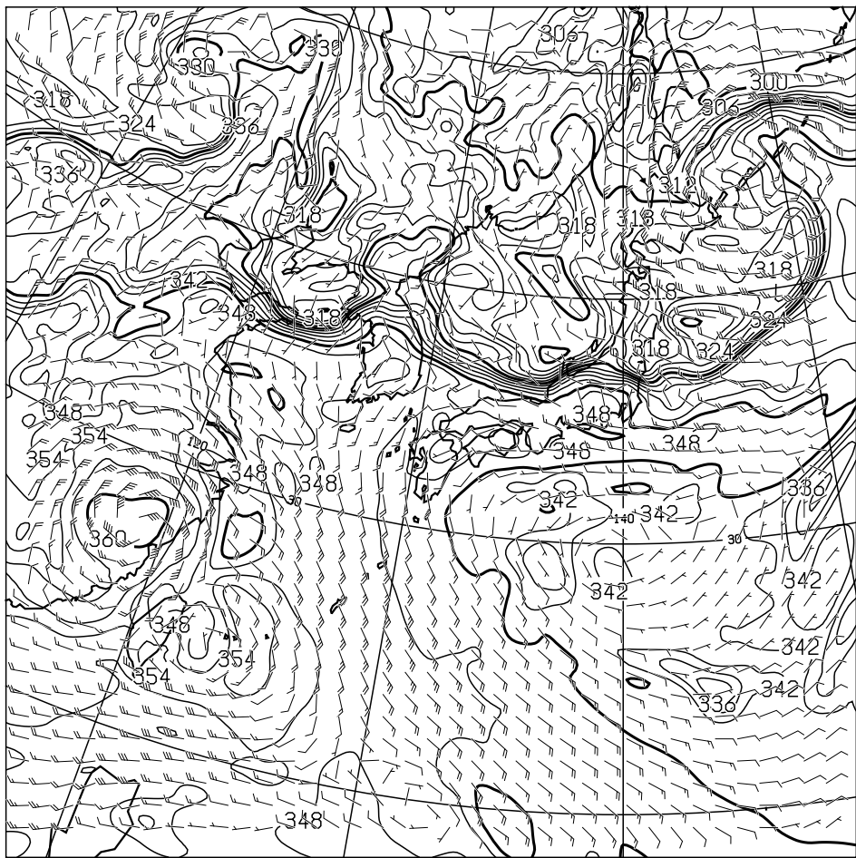
T=48 850hPa: E.P.TEMP(K),WIND(KNOTS) VALID 281200UTC
