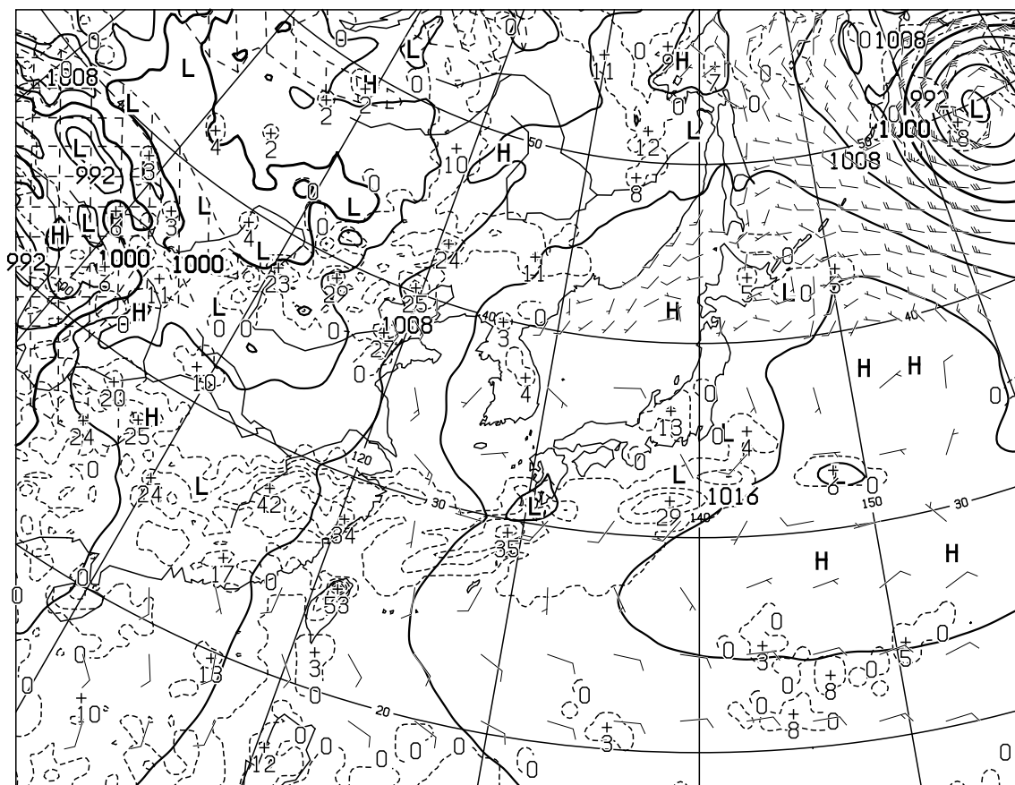
T=24 VALID 291200UTC SURFACE PRESS(hPa),PRECIP(MM) (12-24) WIND ARROW AT SURFACE
