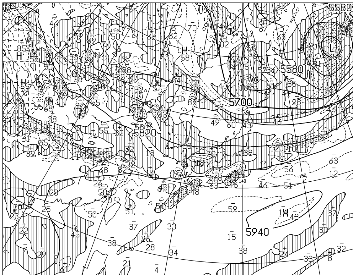
T=12 VALID 290000UTC HEIGHT(M),VORT(10 \times -6/SEC) AT 500hPa
