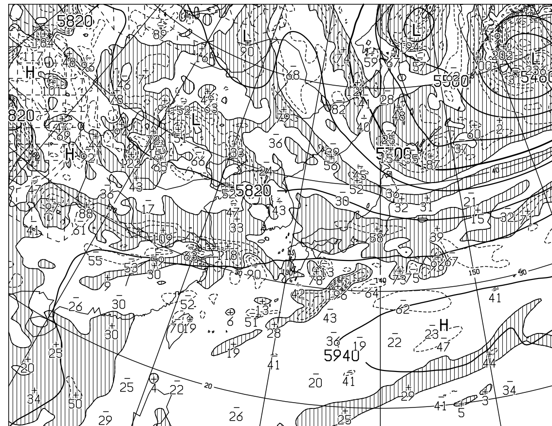
T=24 VALID 291200UTC HEIGHT(M),VORT(10 \times -6/SEC) AT 500hPa
