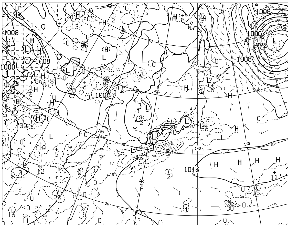
T=12 VALID 290000UTC SURFACE PRESS(hPa),PRECIP(MM) (00-12) WIND ARROW AT SURFACE
