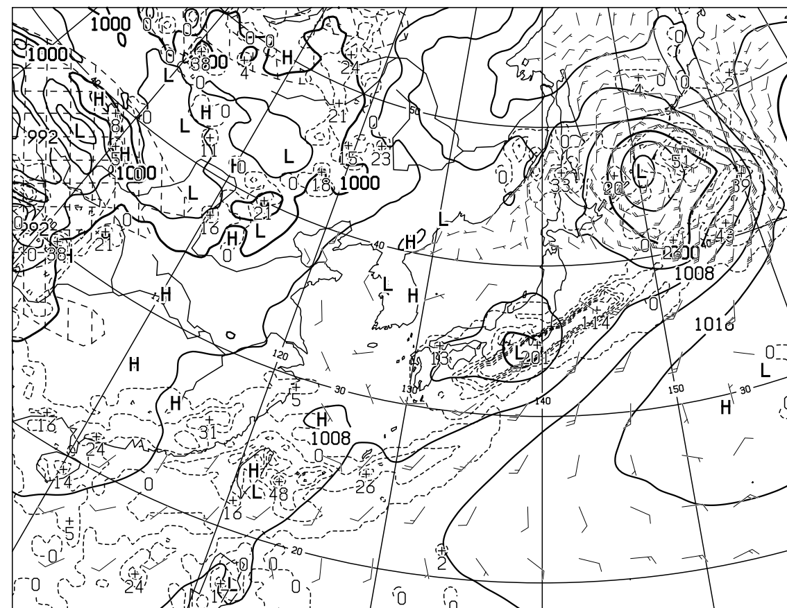
T=24 VALID 271200UTC SURFACE PRESS(hPa),PRECIP(MM) (12-24) WIND ARROW AT SURFACE
