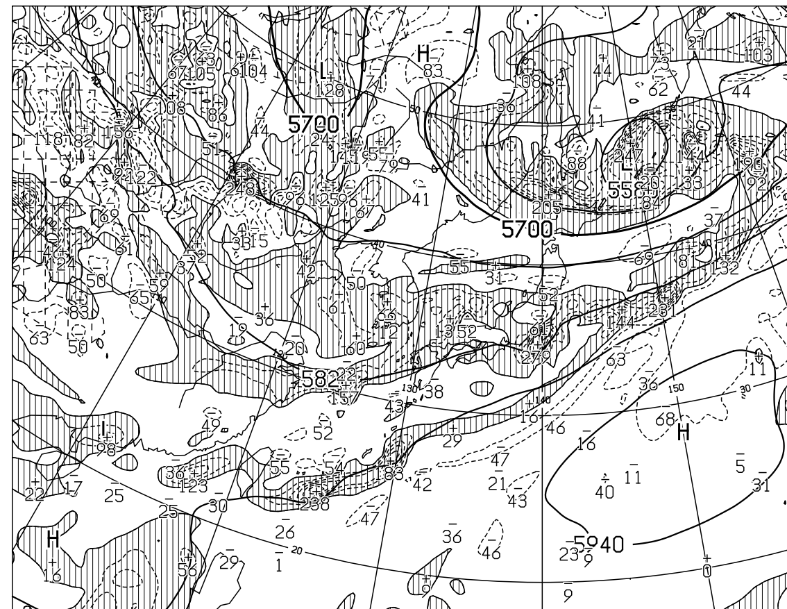
T=24 VALID 271200UTC HEIGHT(M),VORT(10 \times -6/SEC) AT 500hPa
