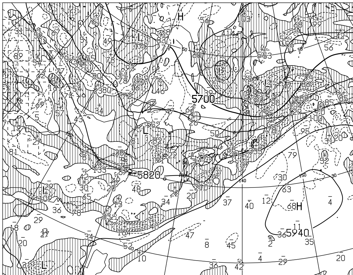
T=12 VALID 270000UTC HEIGHT(M),VORT(10 \times -6/SEC) AT 500hPa
