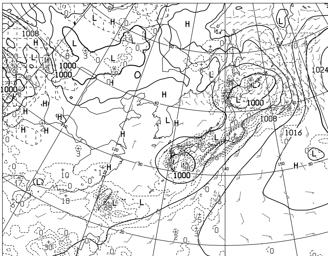
T=12 VALID 270000UTC SURFACE PRESS(hPa),PRECIP(MM) (00-12) WIND ARROW AT SURFACE
