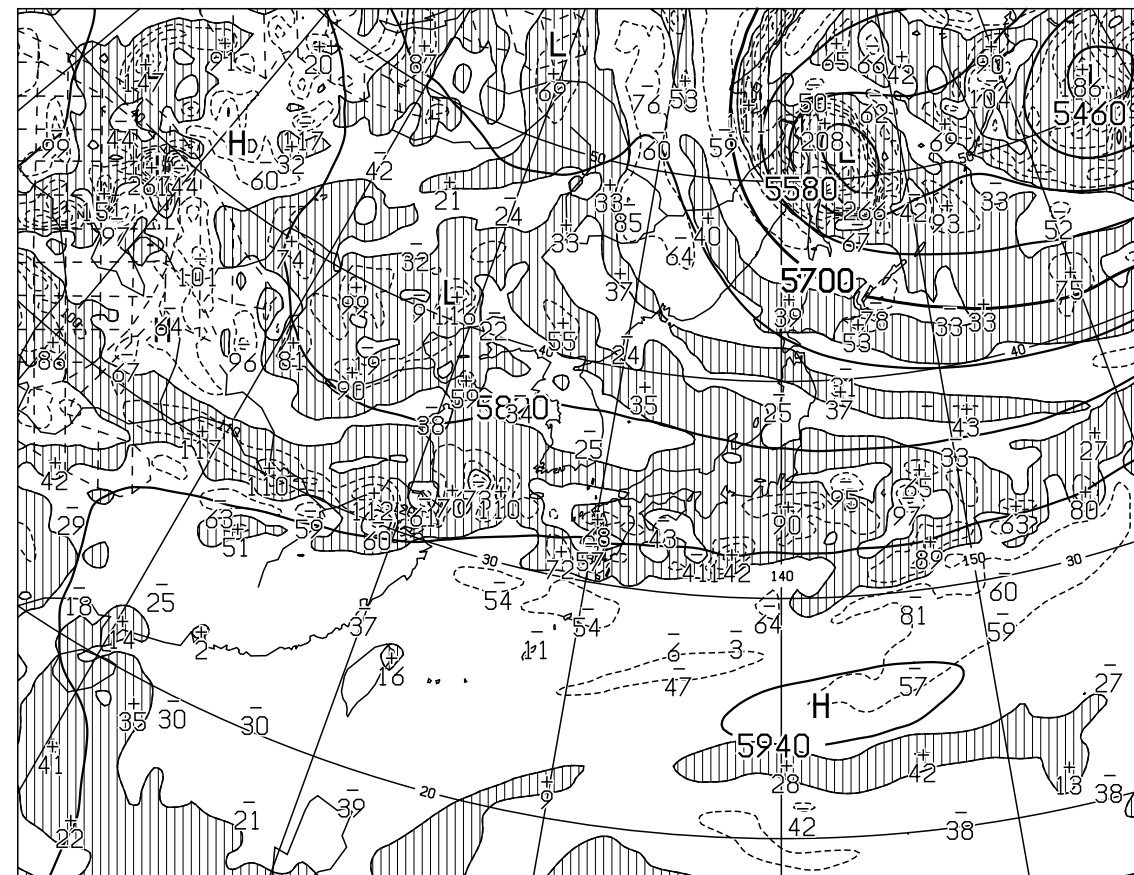
T=24 VALID 301200UTC HEIGHT(M),VORT(10**x-6/SEC) AT 500hPa
