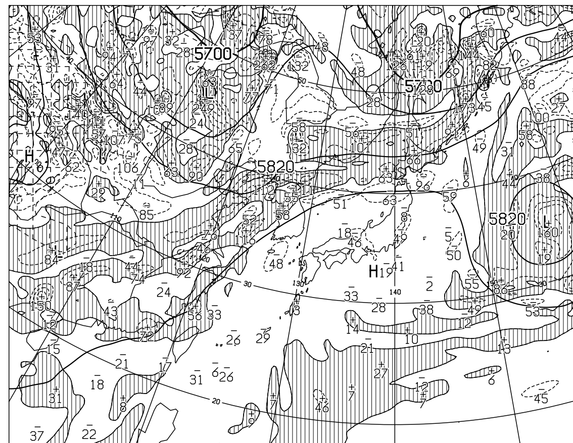
T=24 VALID 201200UTC HEIGHT(M),VORT(10 \times -6/SEC) AT 500hPa
