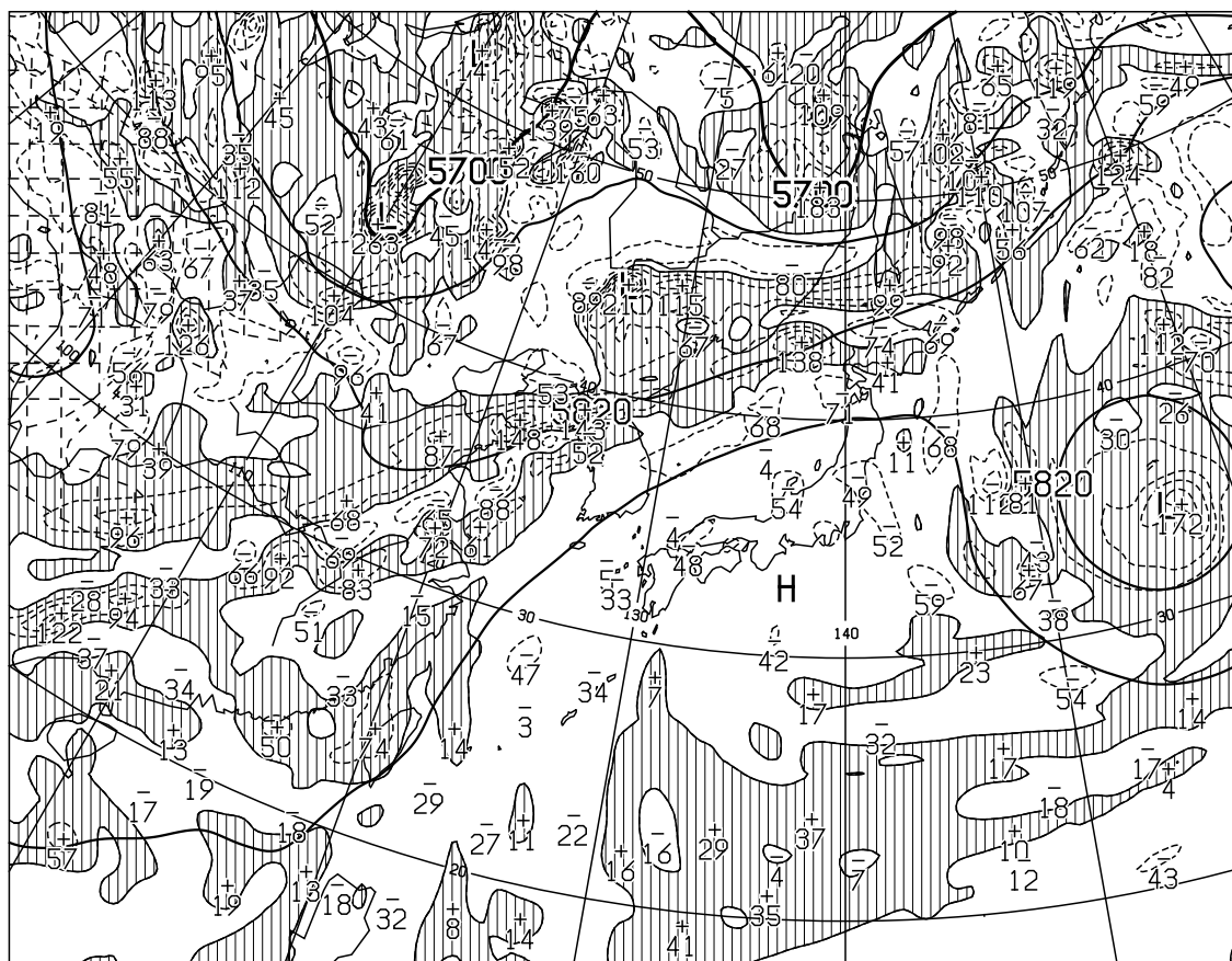
T=12 VALID 200000UTC HEIGHT(M),VORT(10 \times -6/SEC) AT 500hPa
