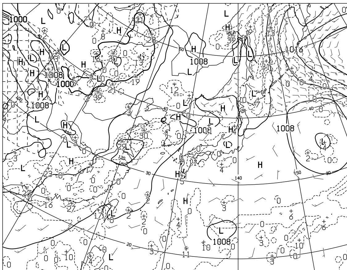
T=12 VALID 200000UTC SURFACE PRESS(hPa),PRECIP(MM) (00-12) WIND ARROW AT SURFACE
