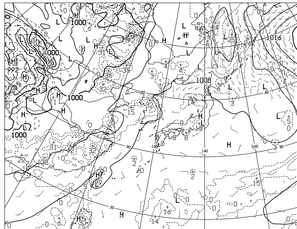
T=24 VALID 201200UTC SURFACE PRESS(hPa),PRECIP(MM) (12-24) WIND ARROW AT SURFACE
