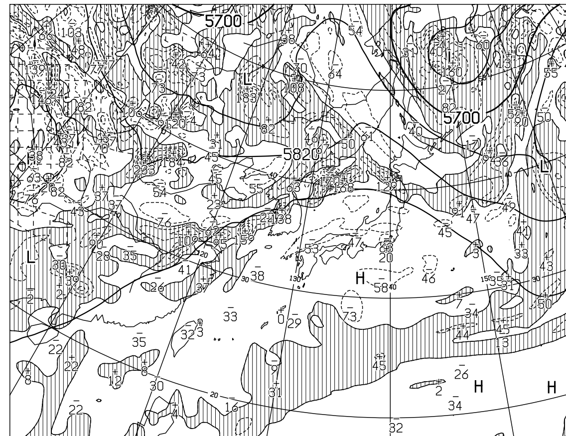
T=24 VALID 211200UTC HEIGHT(M),VORT(10 \times -6/SEC) AT 500hPa
