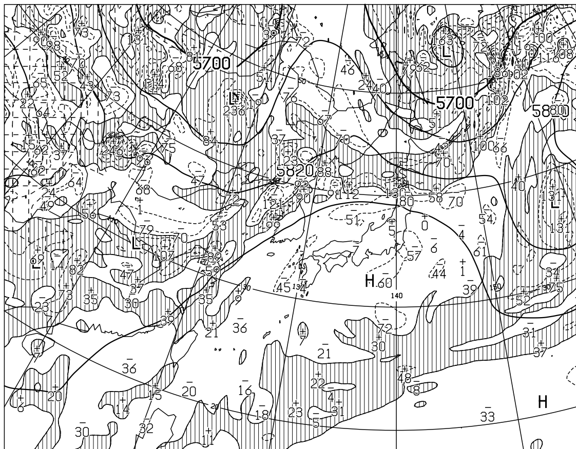
T=12 VALID 210000UTC HEIGHT(M),VORT(10 \times -6/SEC) AT 500hPa
