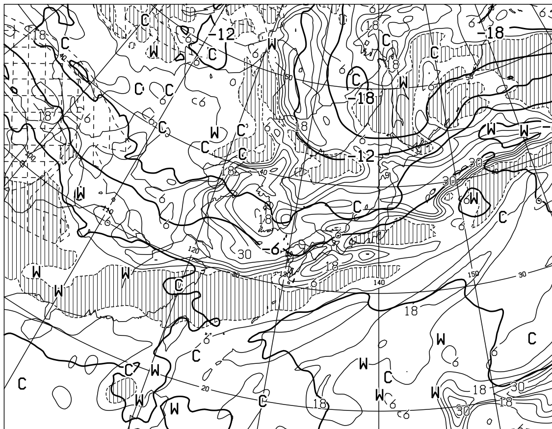
T=12 VALID 280000UTC TEMP ( C ) AT 500hPa T-TD ( C ) AT 700hPa
