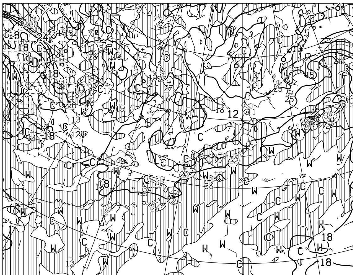
T=12 VALID 280000UTC TEMP ( C ), WIND ARROW AT 850hPa P-VEL (hPa/h) AT 700hPa
