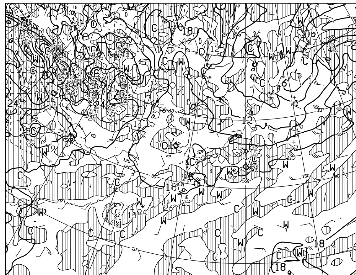
T=24 VALID 281200UTC TEMP ( C ), WIND ARROW AT 850hPa P-VEL (hPa/h) AT 700hPa
