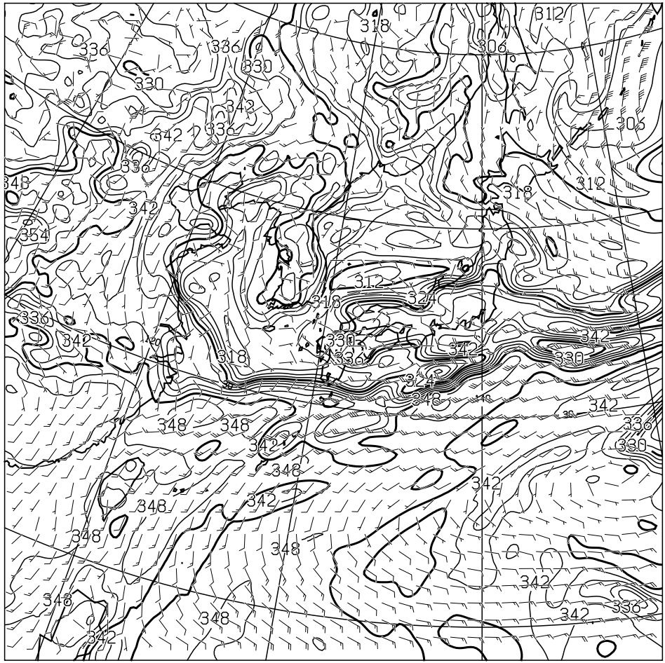
T=24 850hPa: E.P. TEMP(K), WIND(KNOTS) VALID 281200UTC
