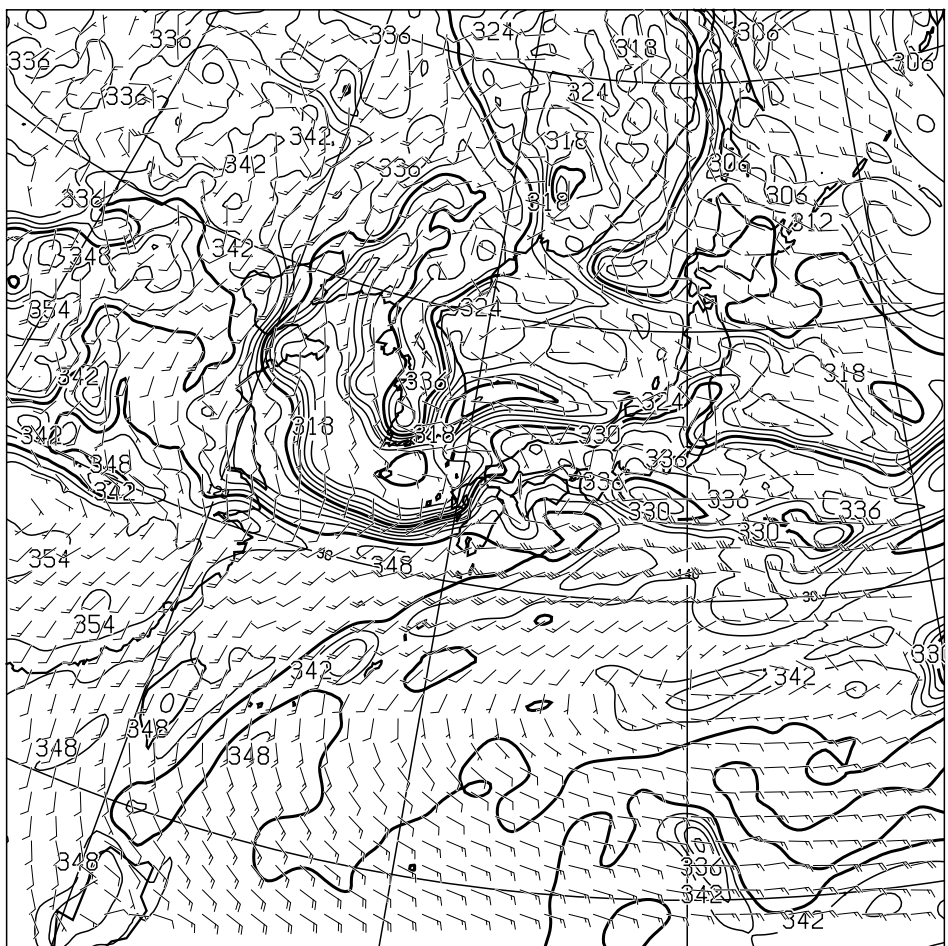
T=48 850hPa: E.P. TEMP(K), WIND(KNOTS) VALID 291200UTC
