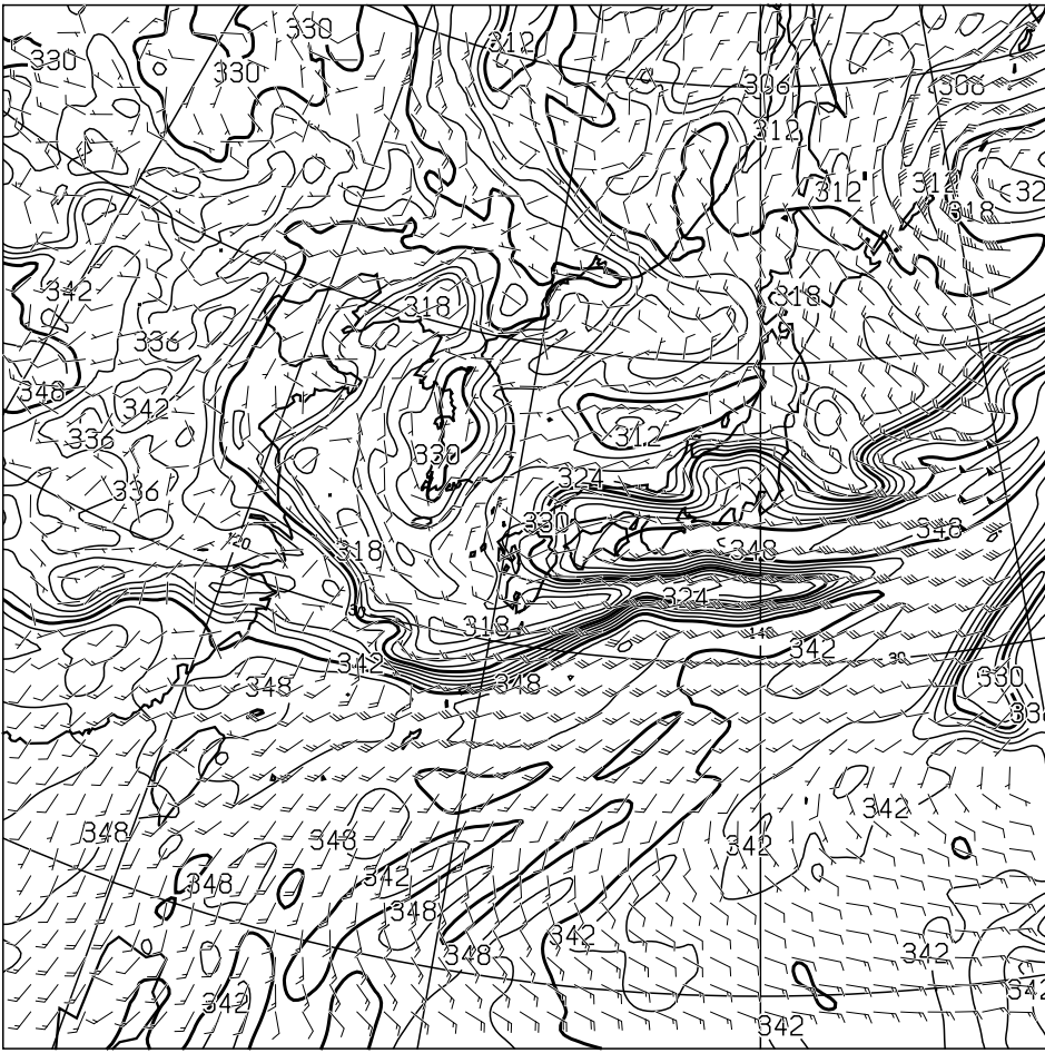
T=12 850hPa: E.P. TEMP(K), WIND(KNOTS) VALID 280000UTC
