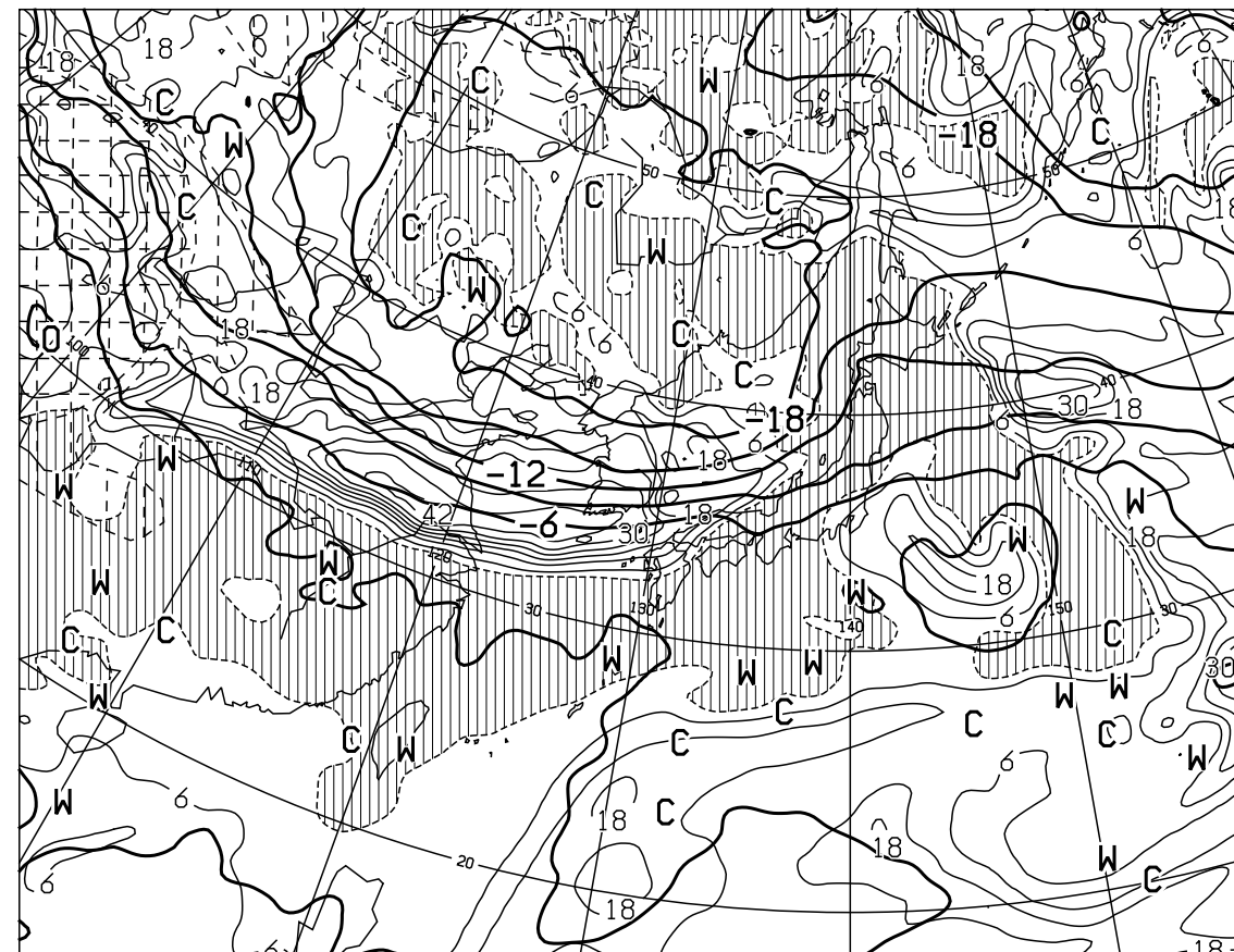
T=24 VALID 081200UTC TEMP (C) AT 500hPa T-TD (C) AT 700hPa
