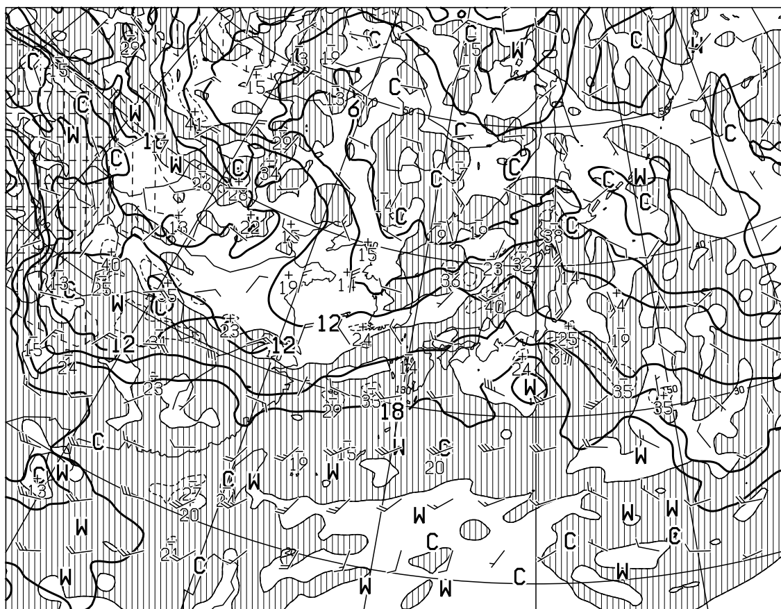
T=12 VALID 080000UTC TEMP (C), WIND ARROW AT 850hPa P-VEL (hPa/H) AT 700hPa
