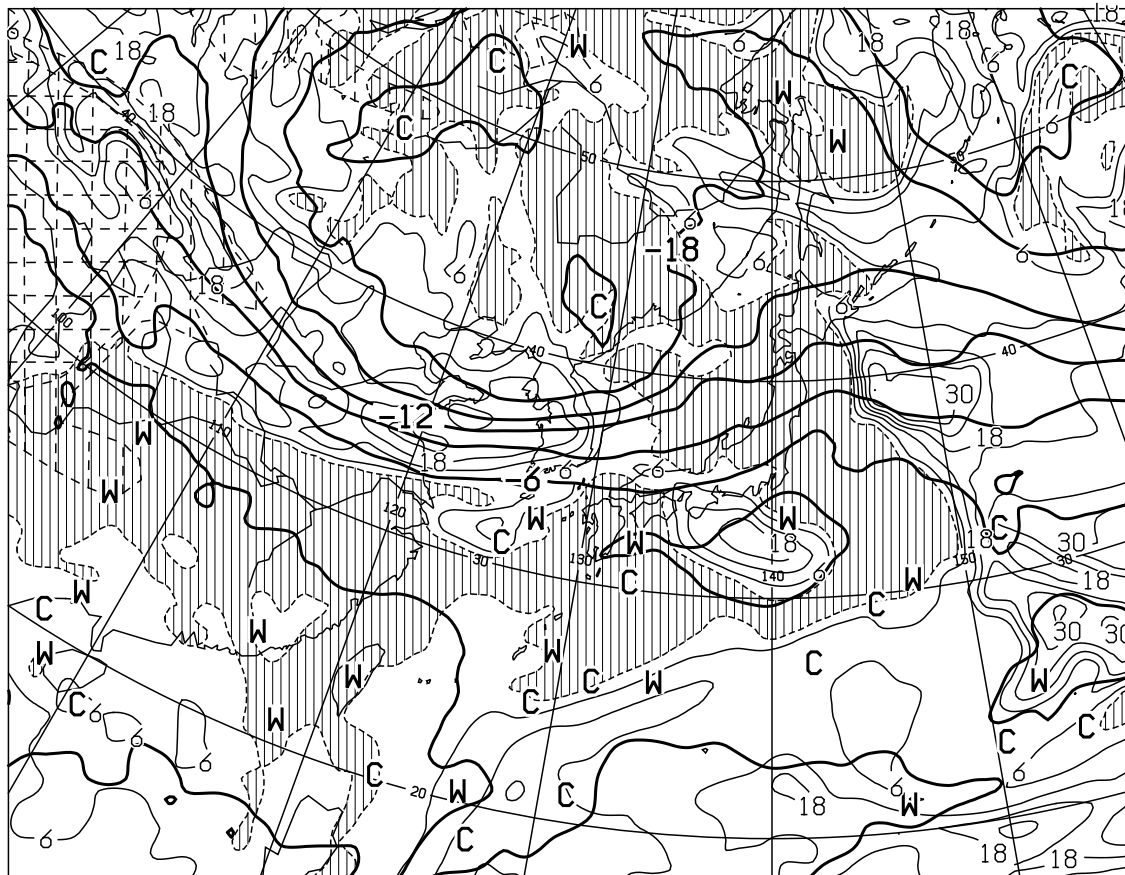
T=12 VALID 080000UTC TEMP (C) AT 500hPa T-TD (C) AT 700hPa
