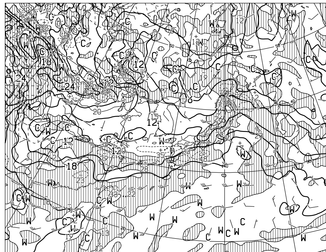
T=24 VALID 081200UTC TEMP (C), WIND ARROW AT 850hPa P-VEL (hPa/H) AT 700hPa
