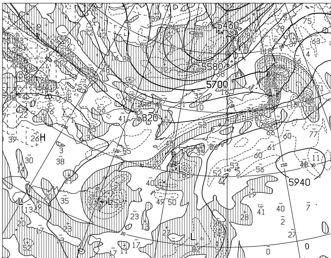
T=12 VALID 080000UTC HEIGHT(M),VORT(10 \times -6/SEC) AT 500hPa
