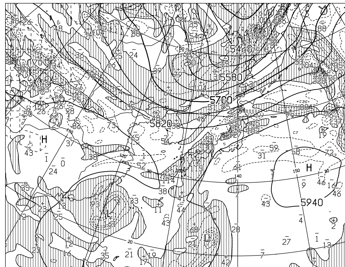
T=24 VALID 081200UTC HEIGHT(M),VORT(10 \times -6/SEC) AT 500hPa
