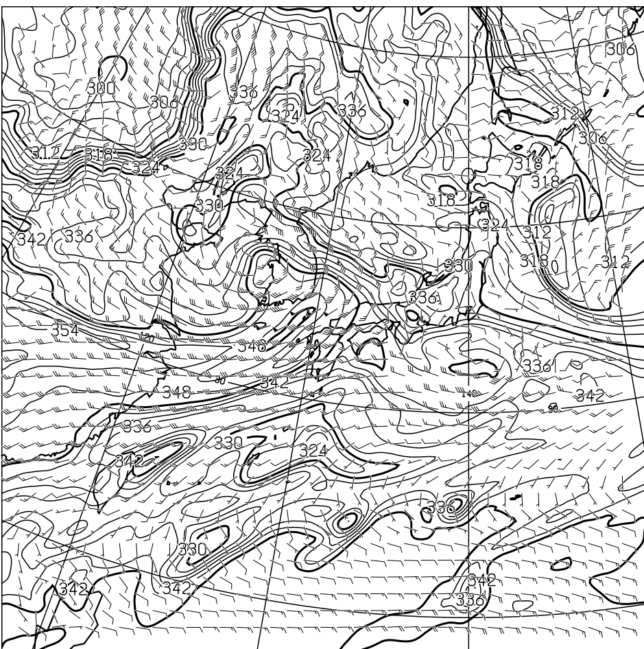
T=36 850hPa: E.P.TEMP(K),WIND(KNOTS) VALID 200000UTC
