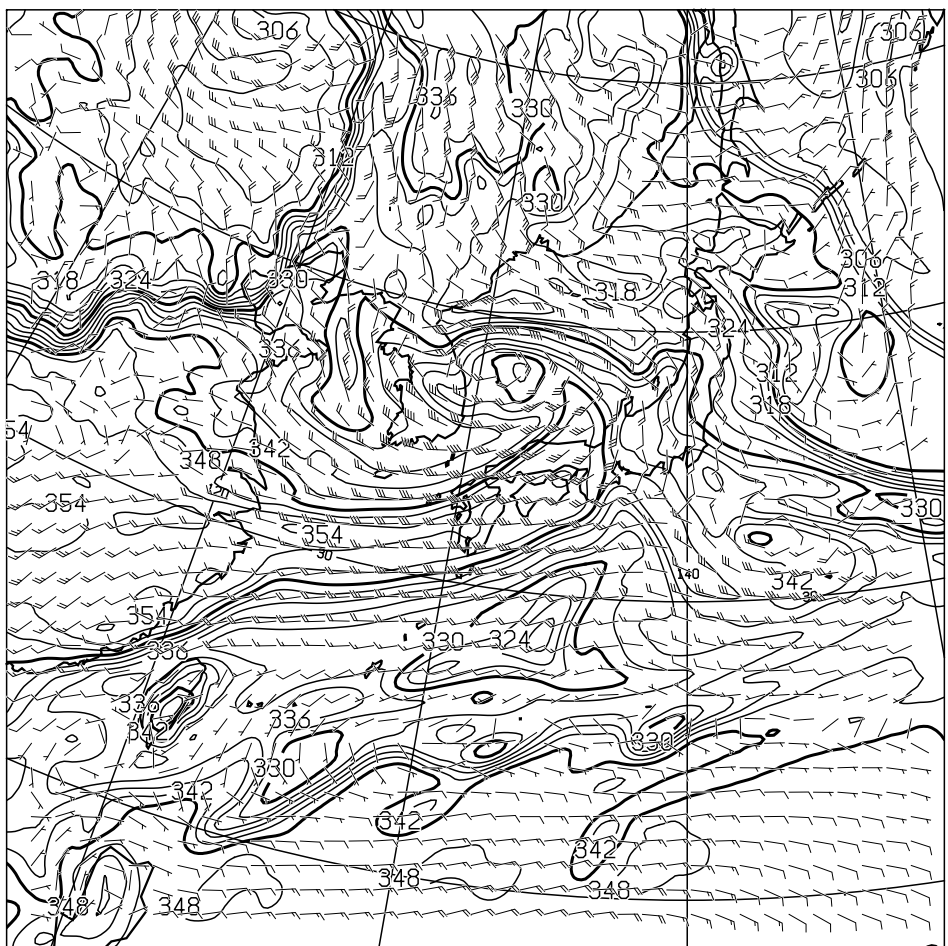
T=48 850hPa: E.P.TEMP(K),WIND(KNOTS) VALID 201200UTC
