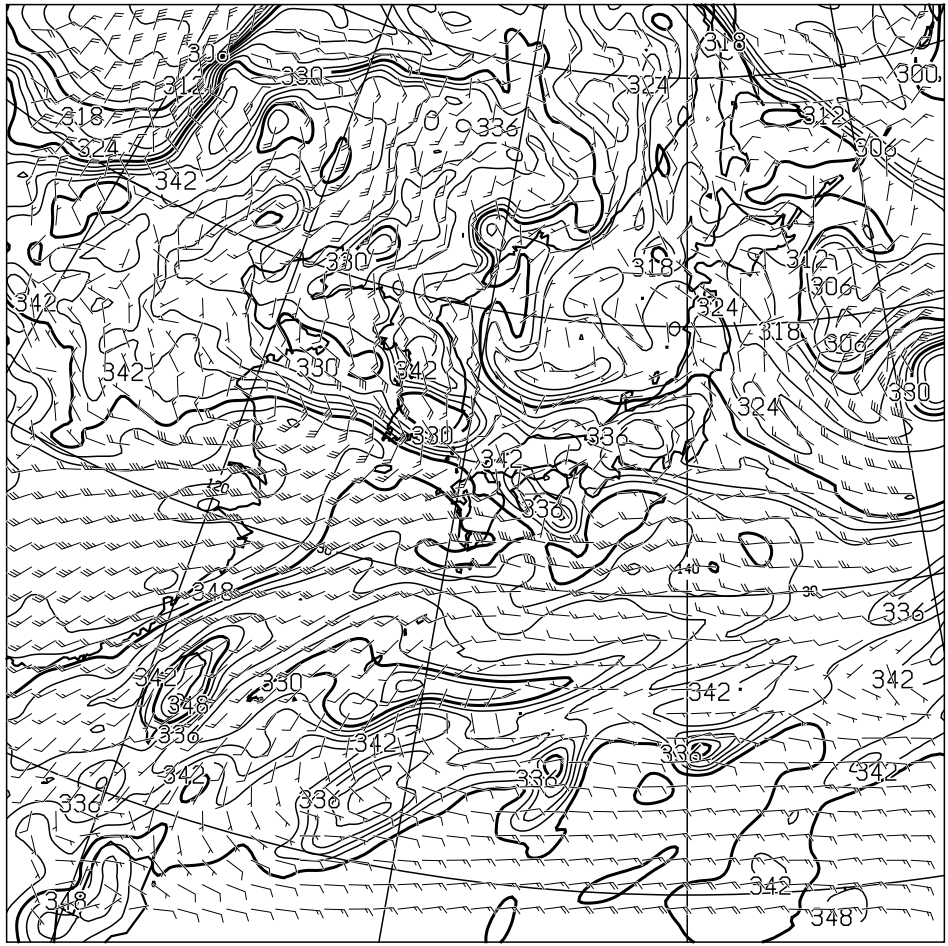
T=24 850hPa: E.P.TEMP(K),WIND(KNOTS) VALID 191200UTC
