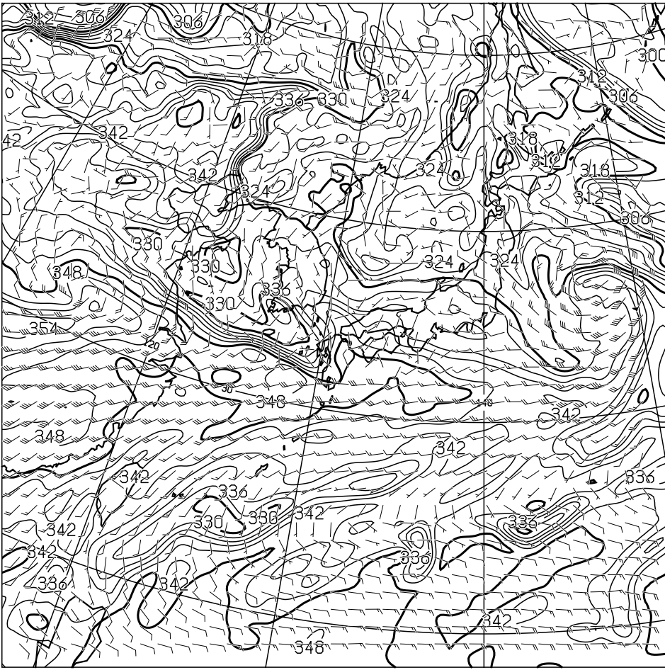
T=12 850hPa: E.P.TEMP(K),WIND(KNOTS) VALID 190000UTC
