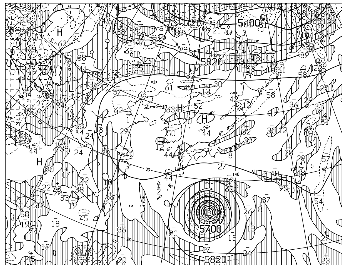
T=24 VALID 051200UTC HEIGHT(M),VORT(10*-6/SEC) AT 500hPa
