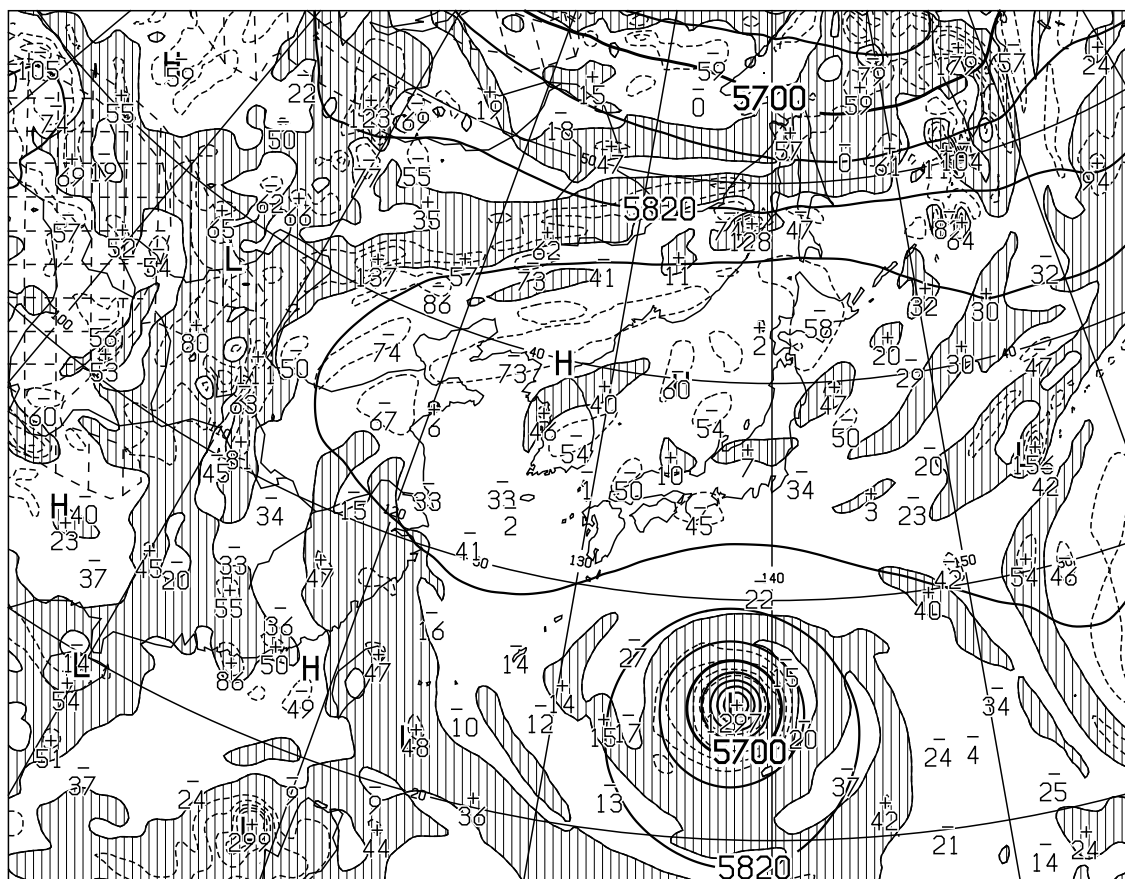
T=12 VALID 050000UTC HEIGHT(M),VORT(10*-6/SEC) AT 500hPa
