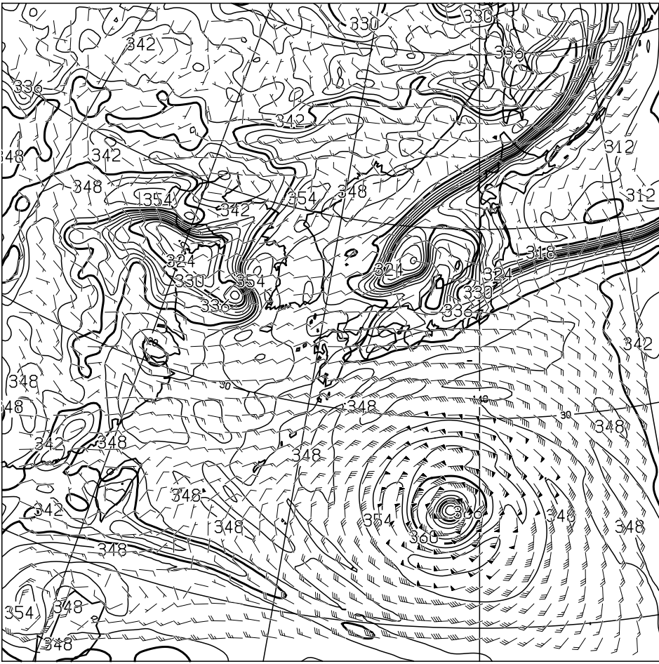
T=12 850hPa: E.P.TEMP(K),WIND(KNOTS) VALID 050000UTC
