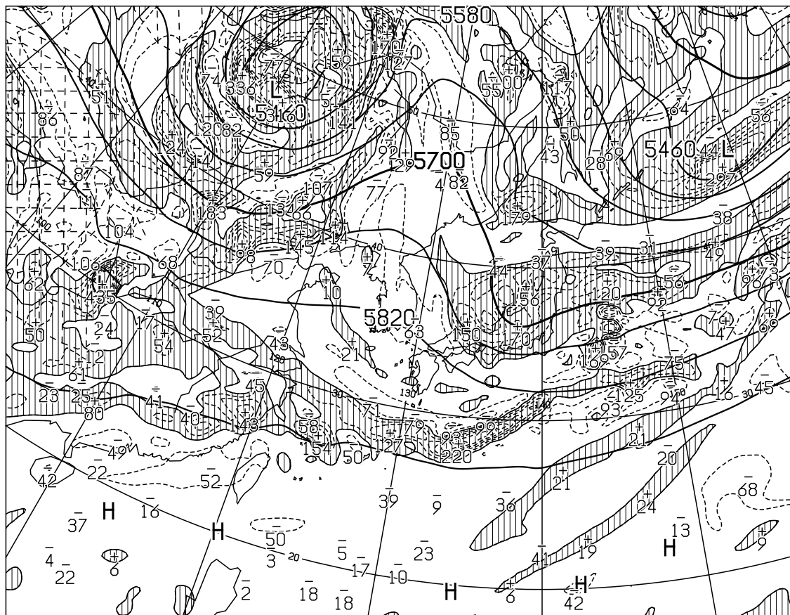
T=12 VALID 220000UTC HEIGHT(M),VORT(10 -6 /SEC) AT 500hPa
