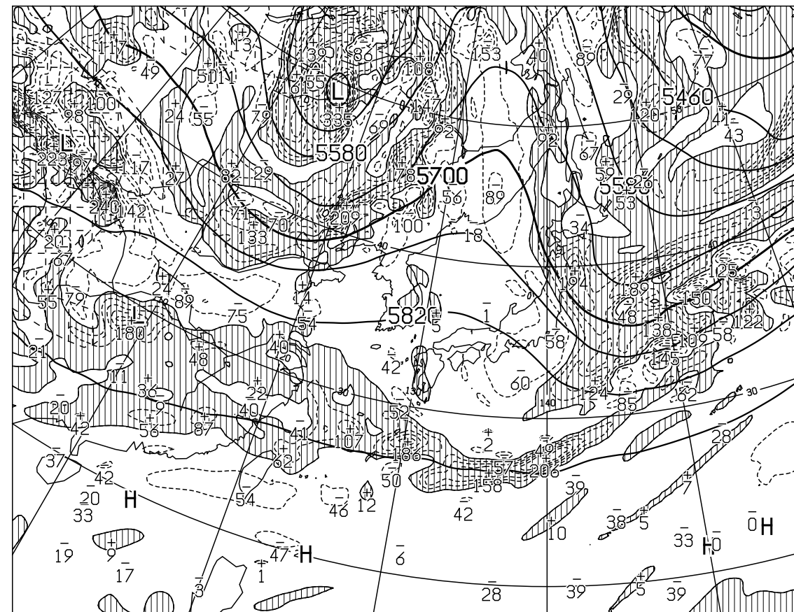
T=24 VALID 221200UTC HEIGHT(M),VORT(10 -6 /SEC) AT 500hPa
