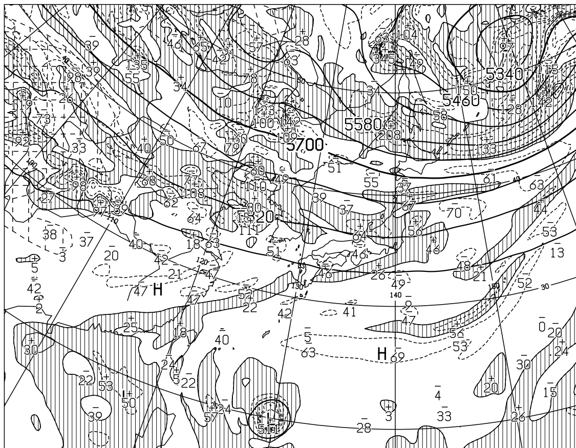
T=12 VALID 250000UTC HEIGHT(M),VORT(10 \times -6/SEC) AT 500hPa
