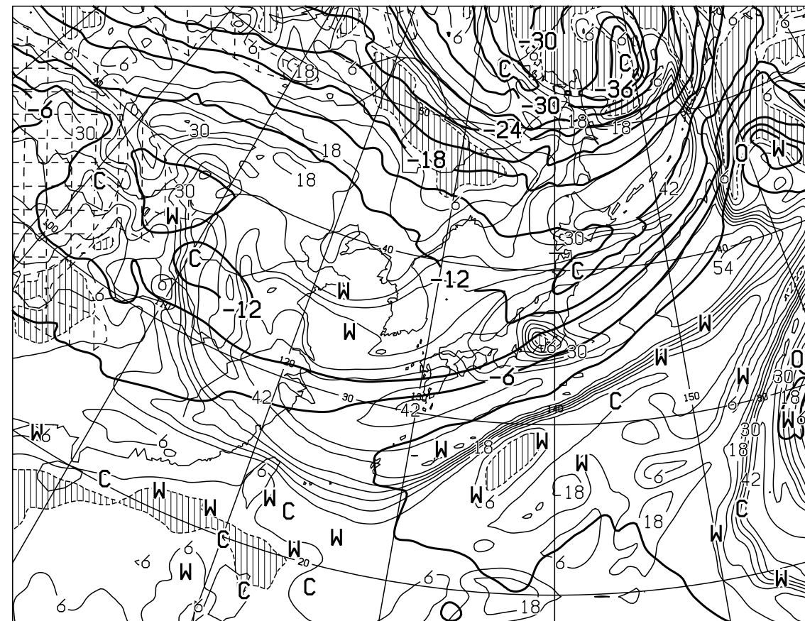
T=24 VALID 071200UTC TEMP( C) AT 500hPa T-TD( C) AT 700hPa
