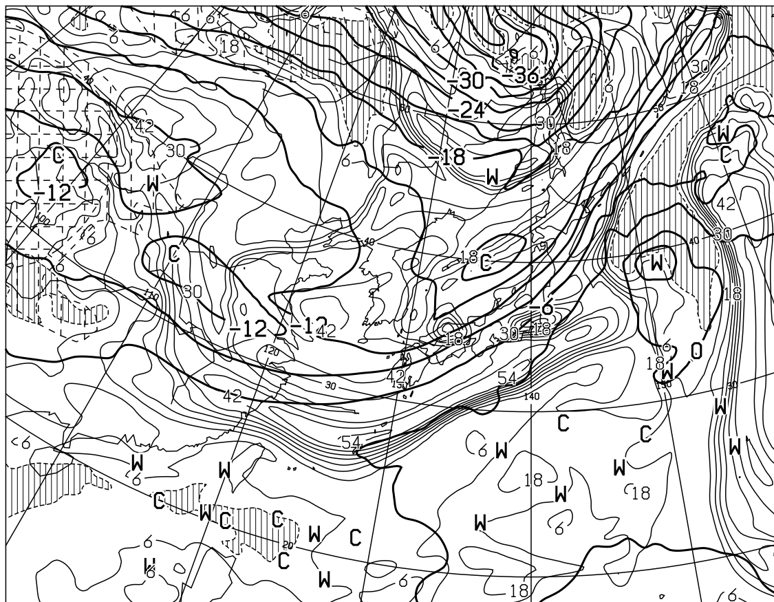
T=12 VALID 070000UTC TEMP( C) AT 500hPa T-TD( C) AT 700hPa
