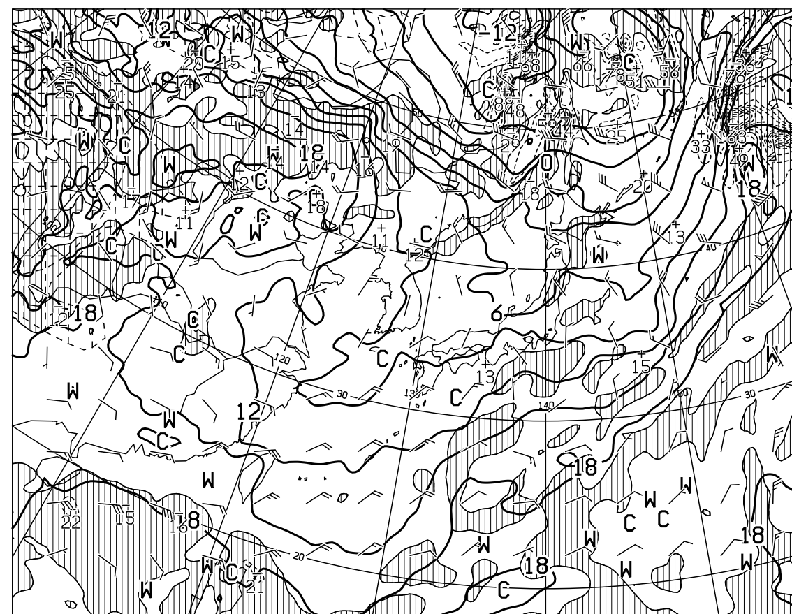
T=24 VALID 071200UTC TEMP( C), WIND ARROW AT 850hPa P-VEL(hPa/H) AT 700hPa
