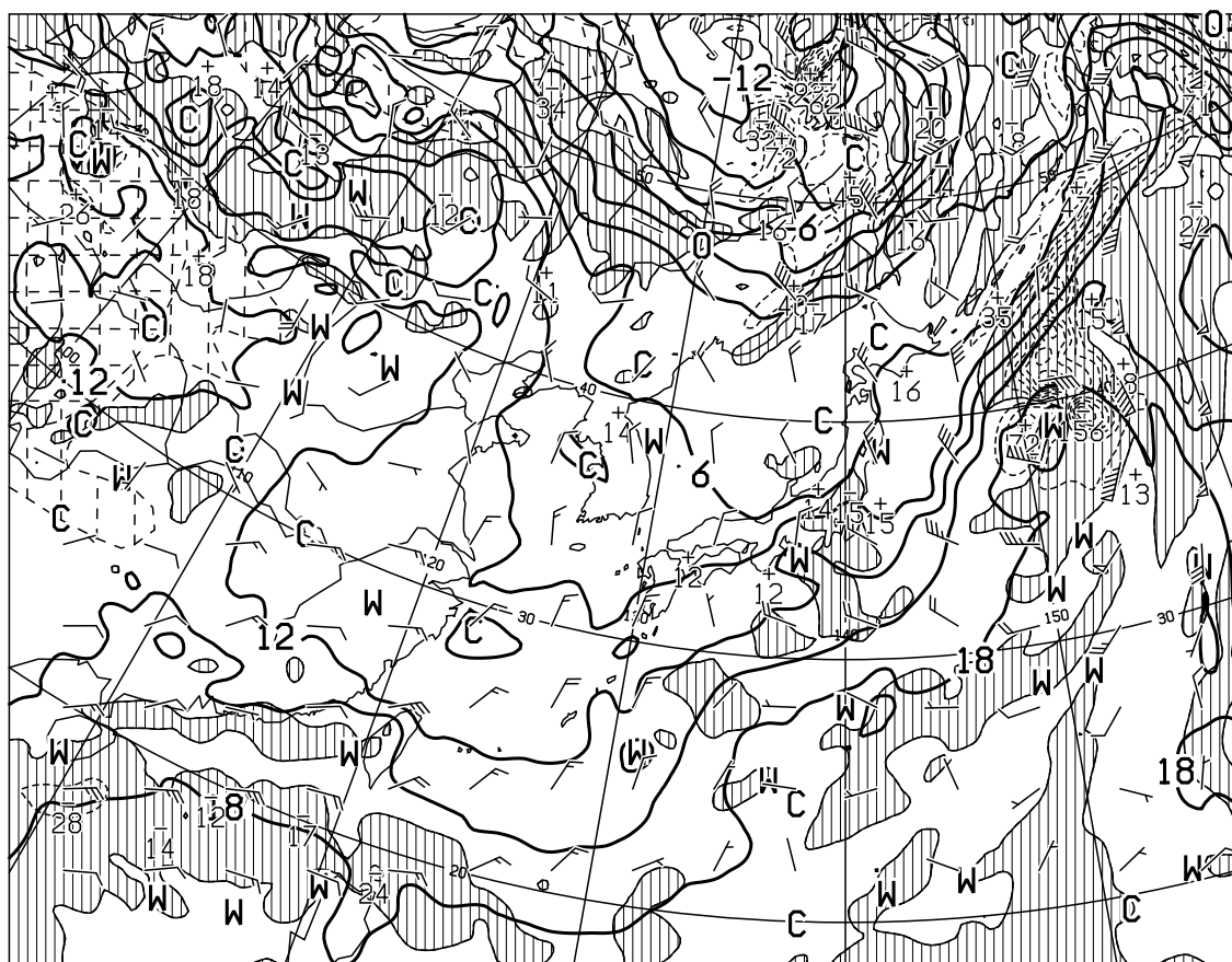
T=12 VALID 070000UTC TEMP( C), WIND ARROW AT 850hPa P-VEL(hPa/H) AT 700hPa
