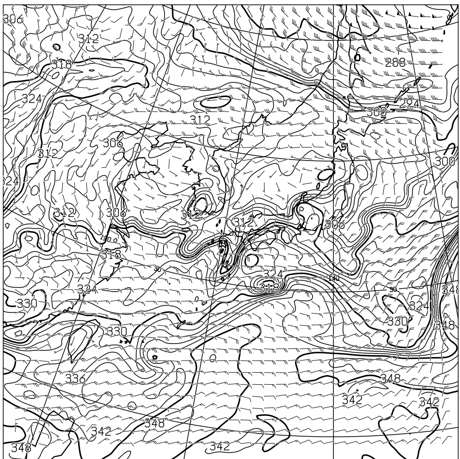
T=48 850hPa: E.P.TEMP(K),WIND(KNOTS) VALID 081200UTC
