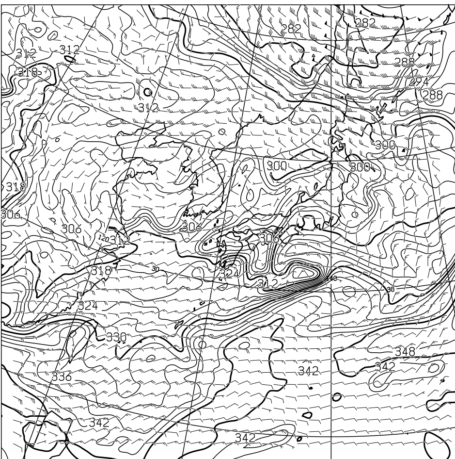
T=36 850hPa: E.P.TEMP(K),WIND(KNOTS) VALID 080000UTC
