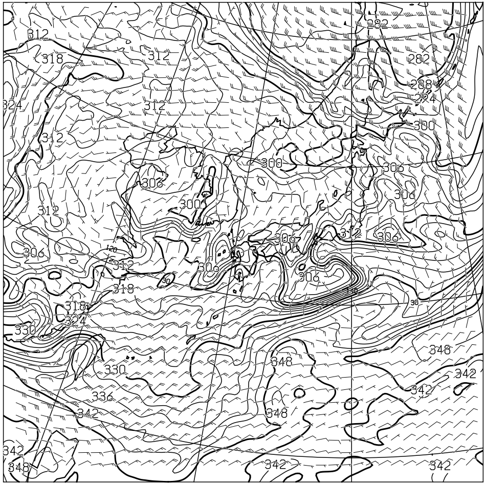
T=24 850hPa: E.P.TEMP(K),WIND(KNOTS) VALID 071200UTC
