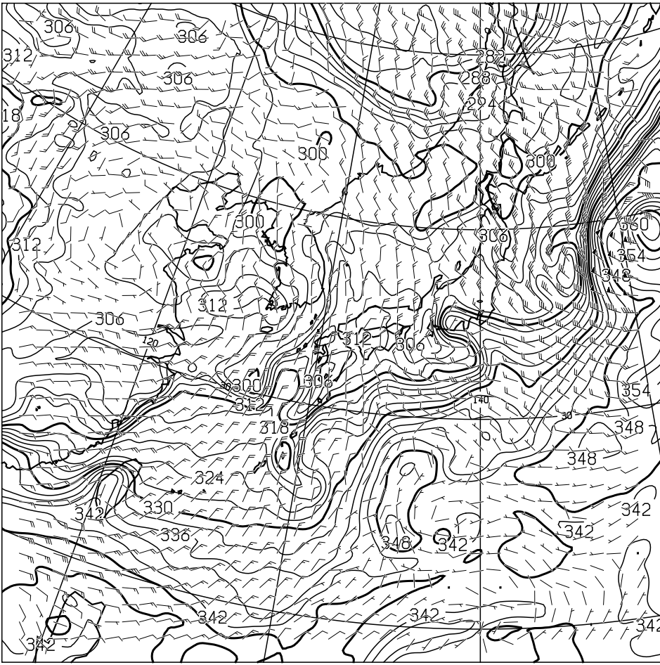
T=12 850hPa: E.P.TEMP(K),WIND(KNOTS) VALID 070000UTC
