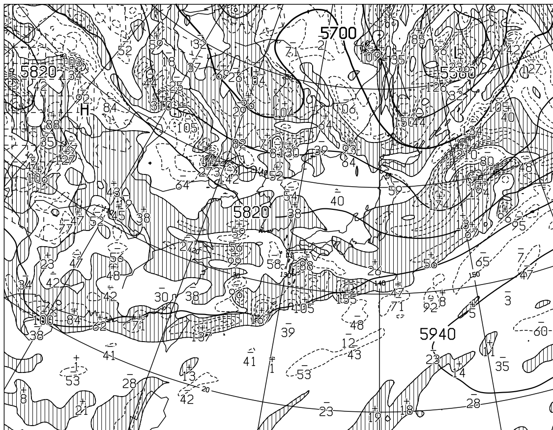
T=12 VALID 160000UTC HEIGHT(M),VORT(10××-6/SEC) AT 500hPa
