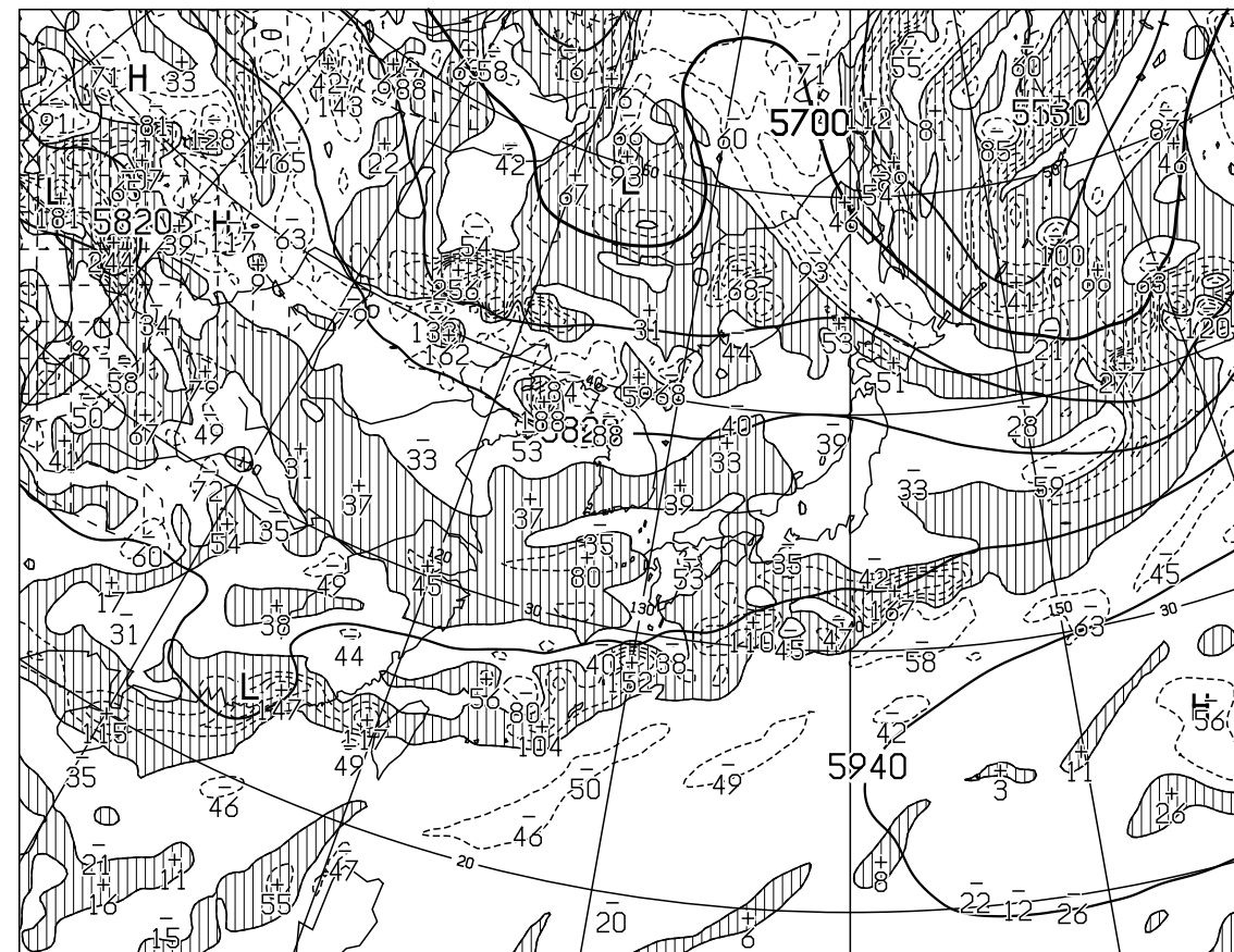
T=24 VALID 161200UTC HEIGHT(M),VORT(10××-6/SEC) AT 500hPa
