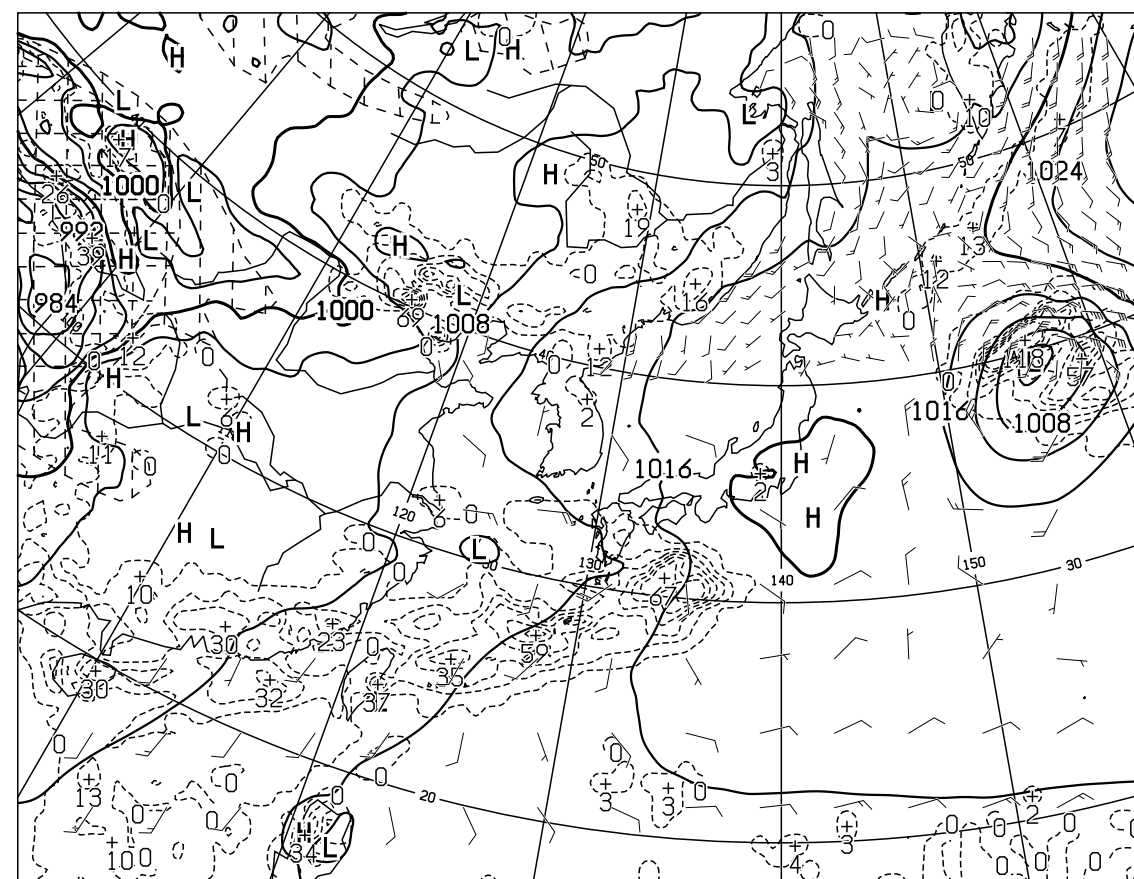
T=24 VALID 161200UTC SURFACE PRESS(hPa),PRECIP(MM) (12-24) WIND ARROW AT SURFACE
