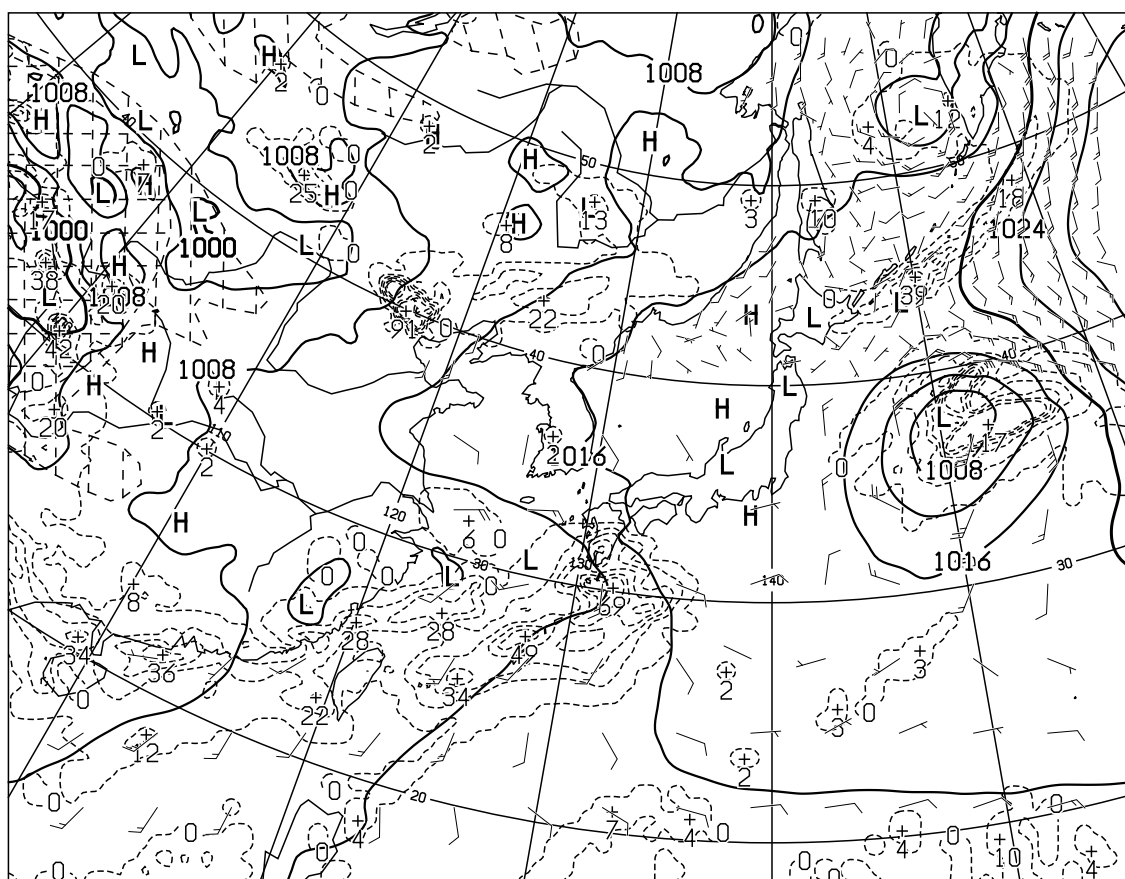
T=12 VALID 160000UTC SURFACE PRESS(hPa),PRECIP(MM) (00-12) WIND ARROW AT SURFACE
