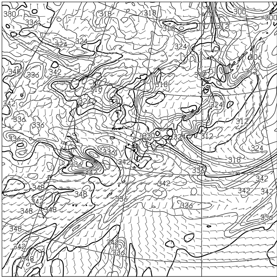
T=24 850hPa: E.P.TEMP(K),WIND(KNOTS) VALID 161200UTC
