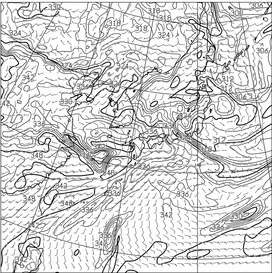
T=36 850hPa: E.P.TEMP(K),WIND(KNOTS) VALID 170000UTC
