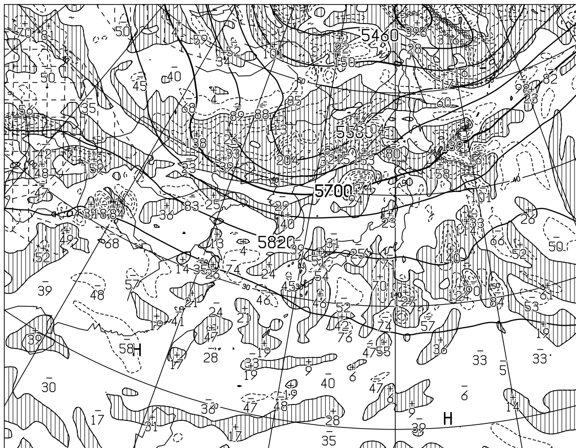
T=12 VALID 280000UTC HEIGHT(M),VORT(10**6/SEC) AT 500hPa
