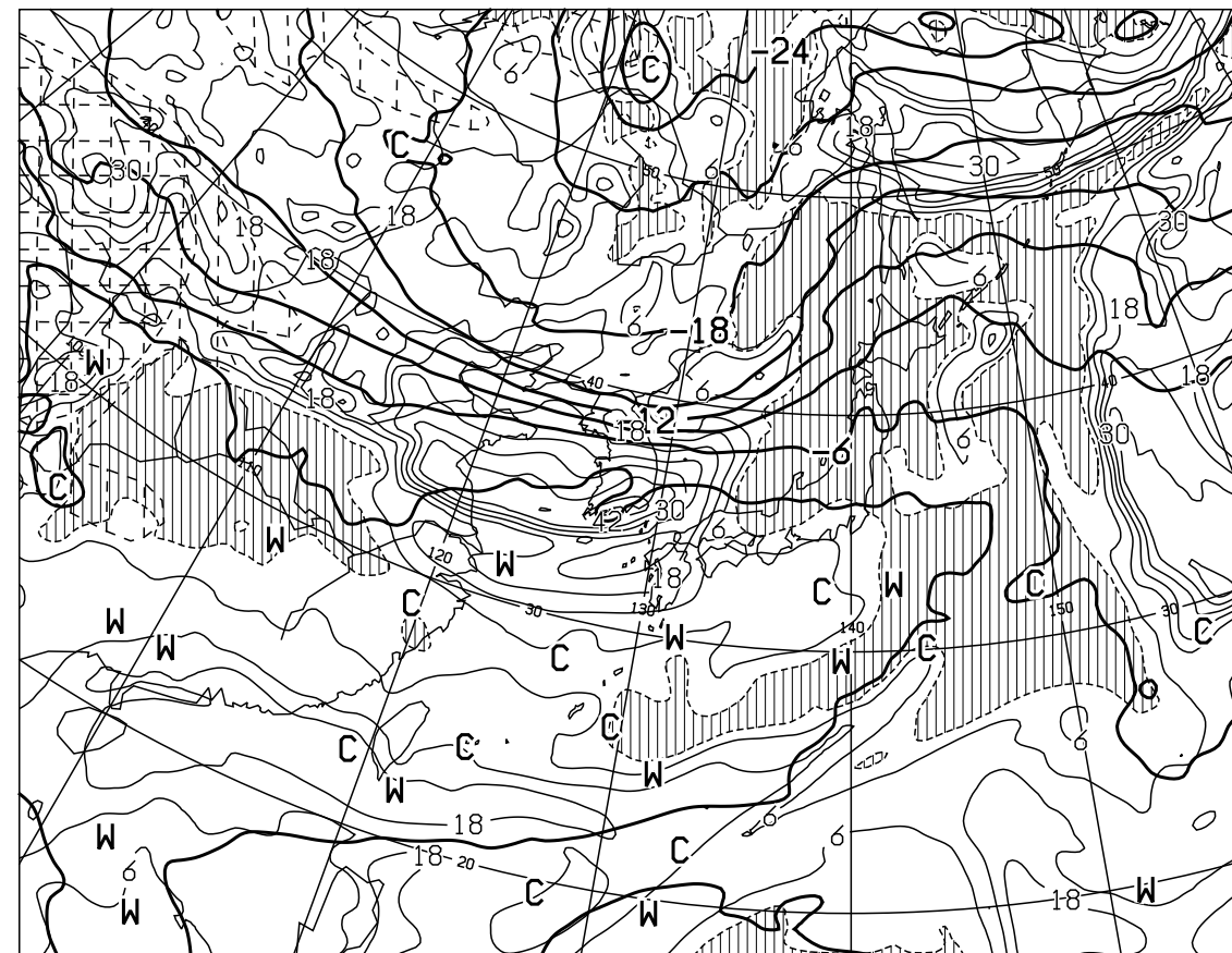
T=24 VALID 281200UTC TEMP (C) AT 500hPa T-D (C) AT 700hPa
