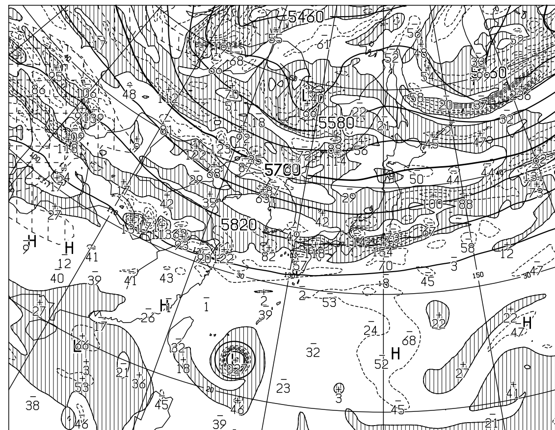
T=24 VALID 261200UTC HEIGHT(M),VORT(10 \times -6/SEC) AT 500hPa
