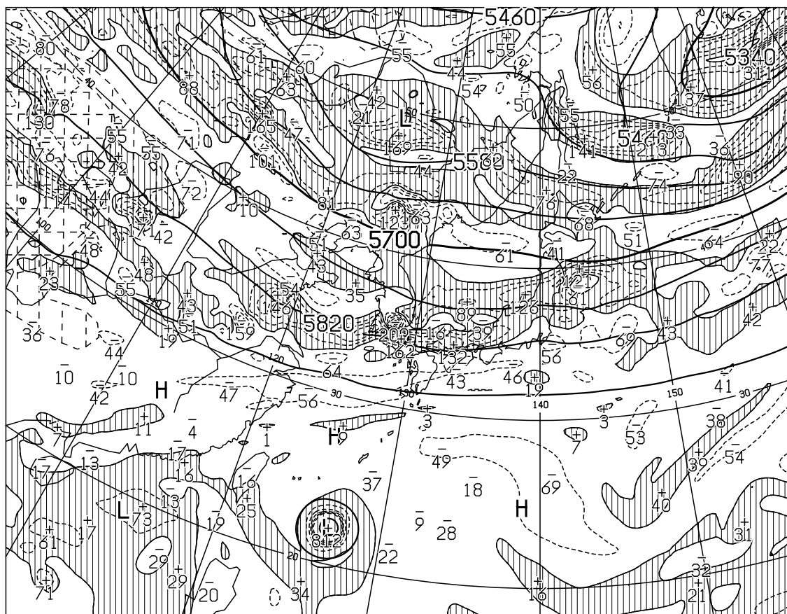
T=12 VALID 260000UTC HEIGHT(M),VORT(10 \times -6/SEC) AT 500hPa
