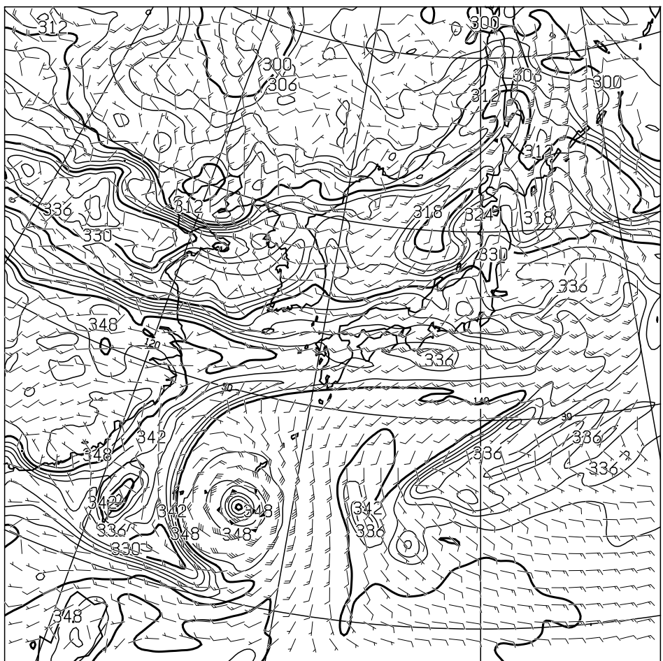
T=48 850hPa: E.P.TEMP(K),WIND(KNOTS) VALID 271200UTC
