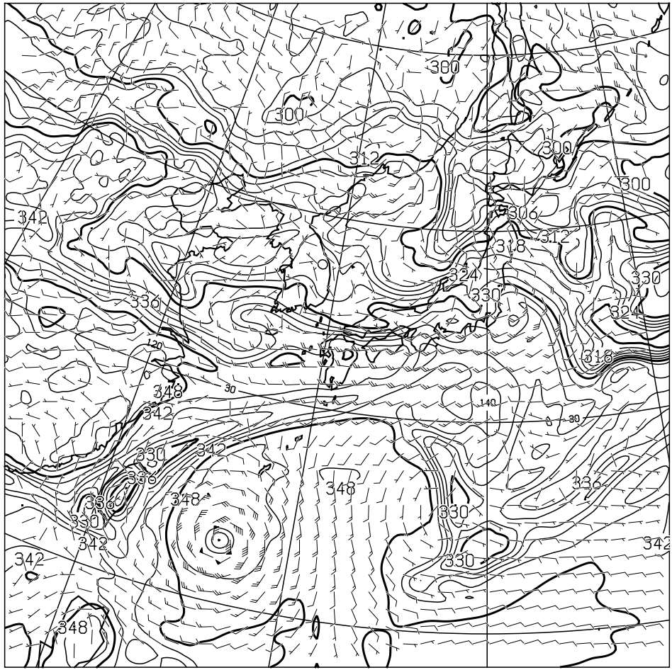
T=24 850hPa: E.P.TEMP(K),WIND(KNOTS) VALID 261200UTC
