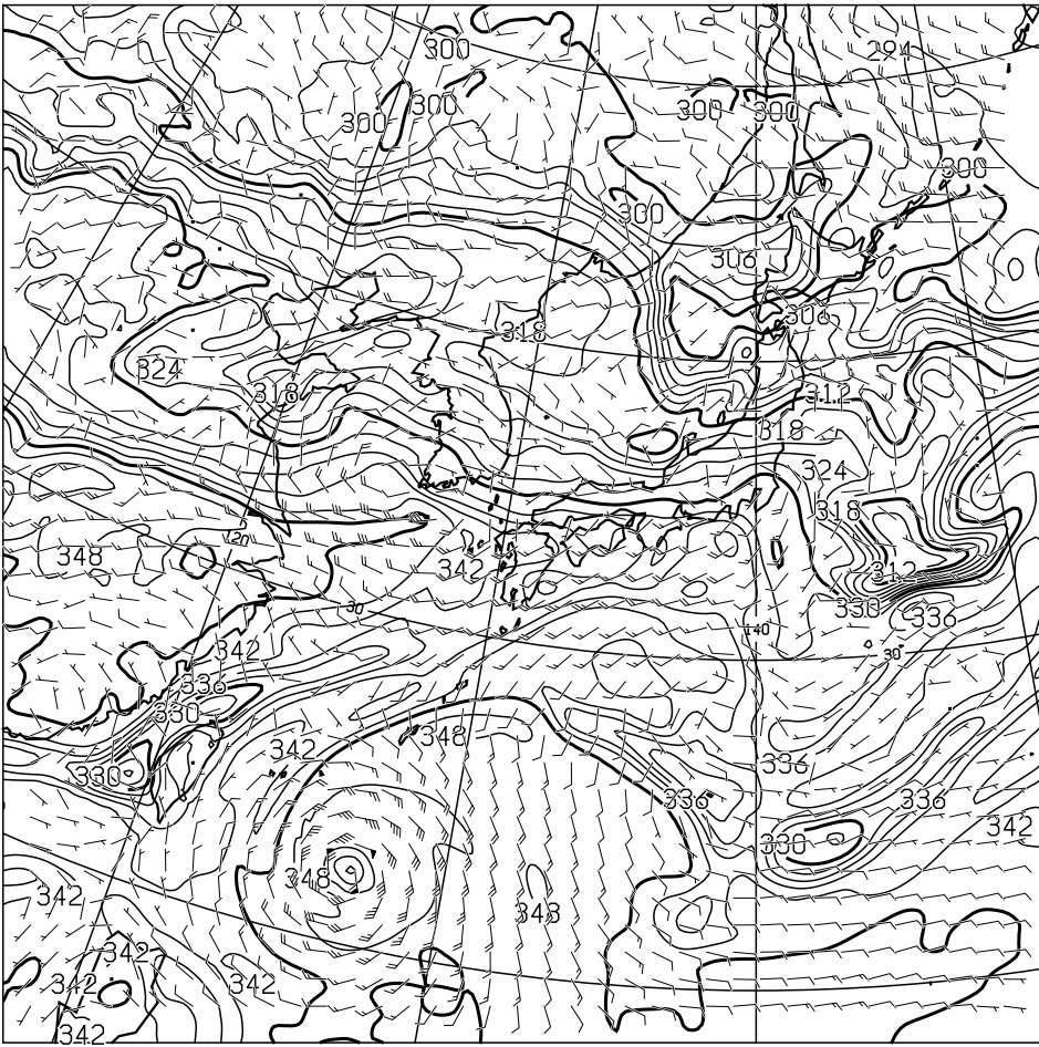
T=12 850hPa: E.P.TEMP(K),WIND(KNOTS) VALID 260000UTC
