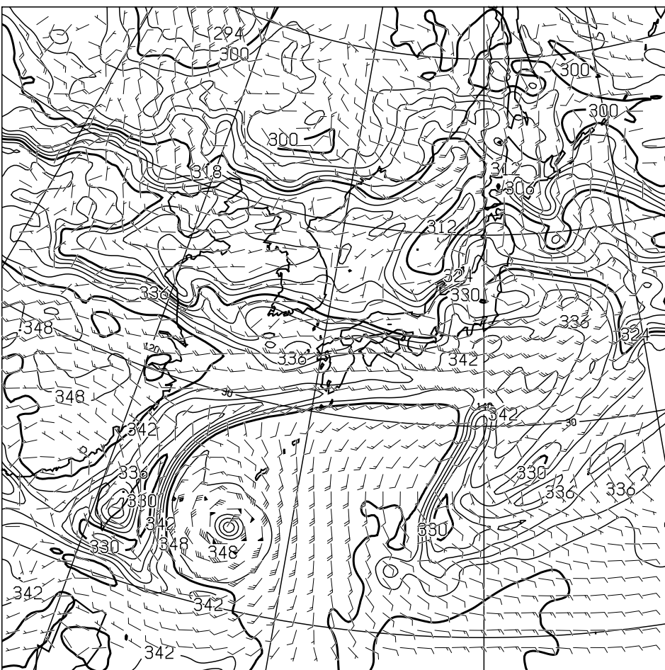
T=36 850hPa: E.P.TEMP(K),WIND(KNOTS) VALID 270000UTC
