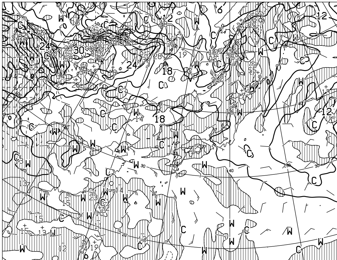
T=24 VALID 191200UTC TEMP (C), WIND ARROW AT 850hPa P-VEL (hPa/h) AT 700hPa
