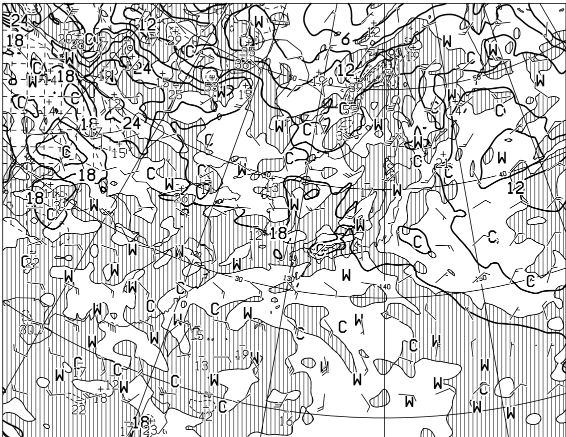
T=12 VALID 190000UTC TEMP (C), WIND ARROW AT 850hPa P-VEL (hPa/h) AT 700hPa
