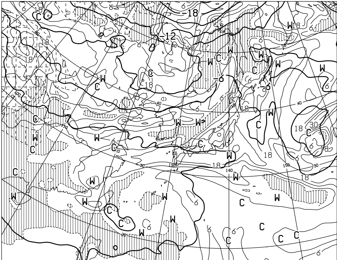
T=12 VALID 190000UTC TEMP (C) AT 500hPa T-TD (C) AT 700hPa
