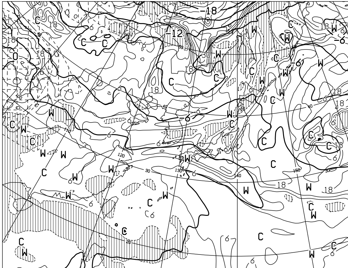
T=24 VALID 191200UTC TEMP (C) AT 500hPa T-TD (C) AT 700hPa
