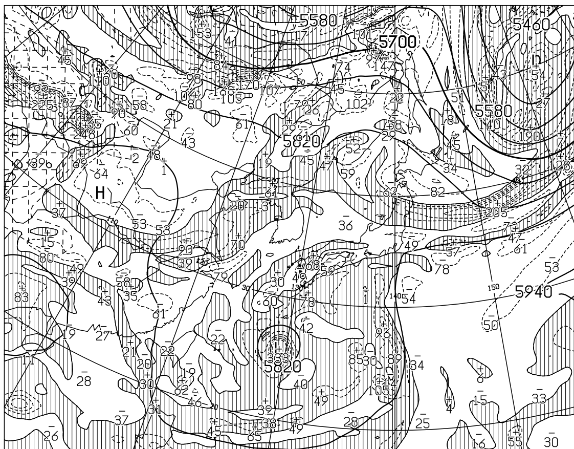
T=12 VALID 060000UTC HEIGHT(M),VORT(10 -6 /SEC) AT 500hPa
