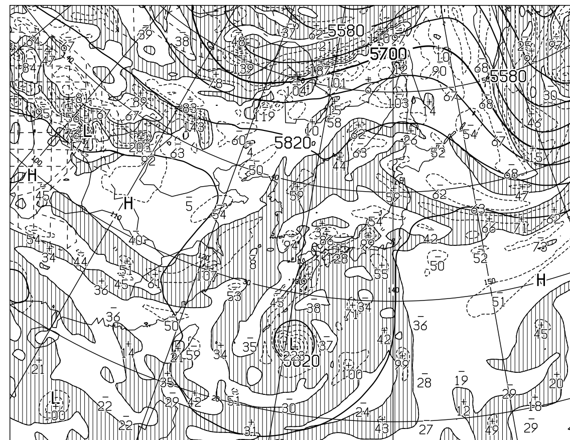
T=24 VALID 061200UTC HEIGHT(M),VORT(10 -6 /SEC) AT 500hPa
