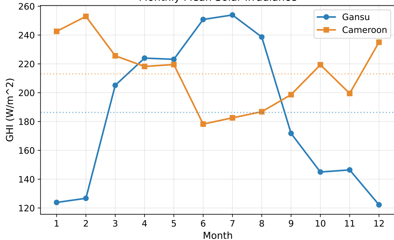
Monthly Mean Solar Irradiance
