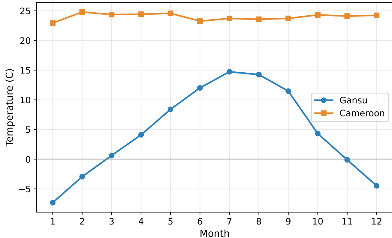
Monthly Mean Temperature
